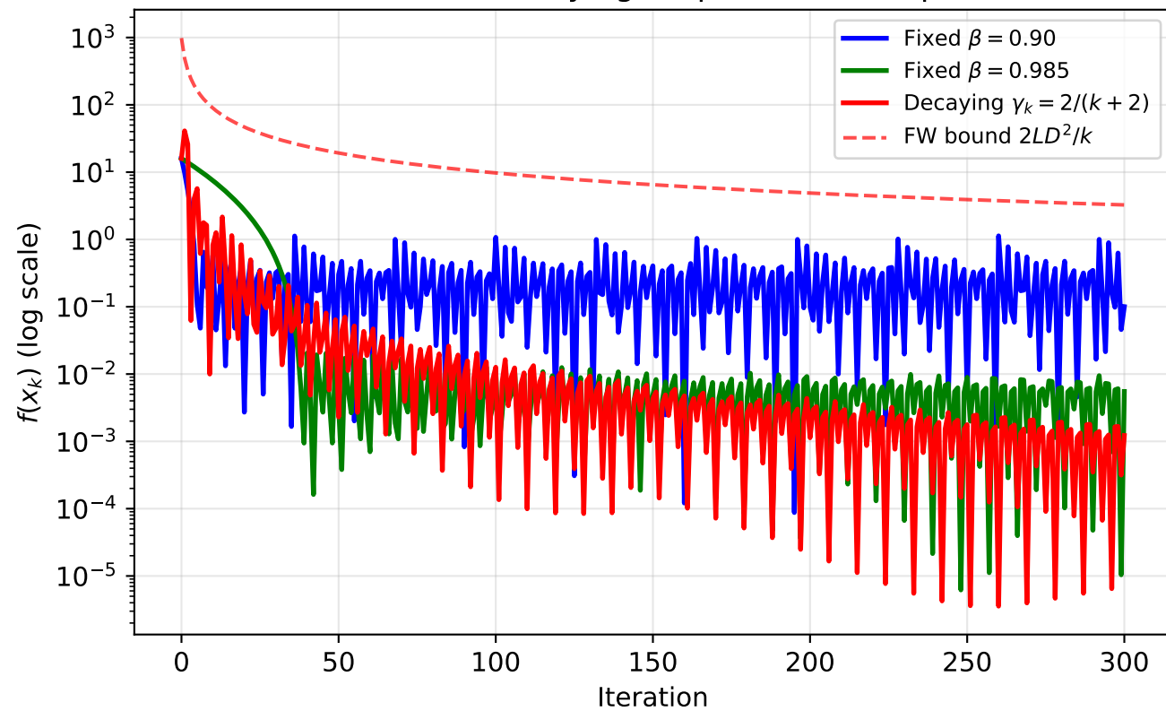
FW: Fixed vs.\ Decaying Step — Interior Optimum
