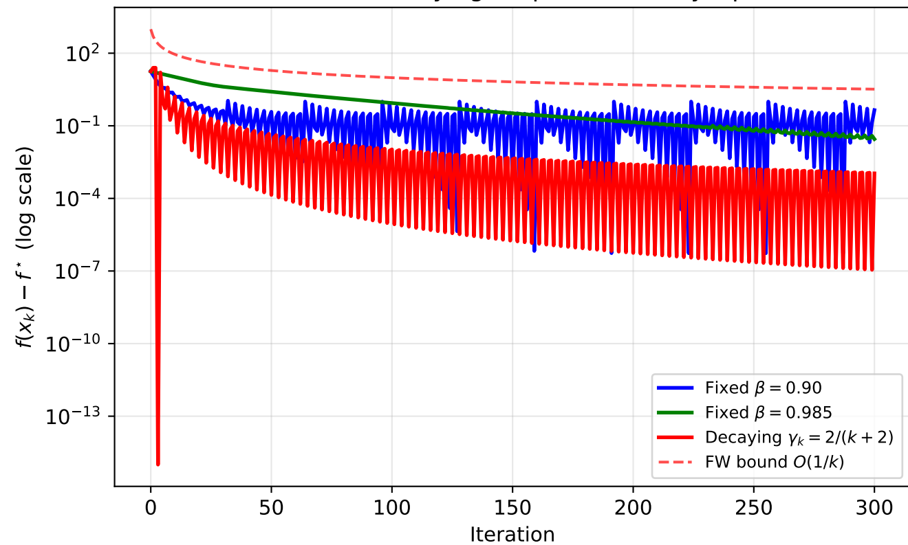
FW: Fixed vs.\ Decaying Step — Boundary Optimum
