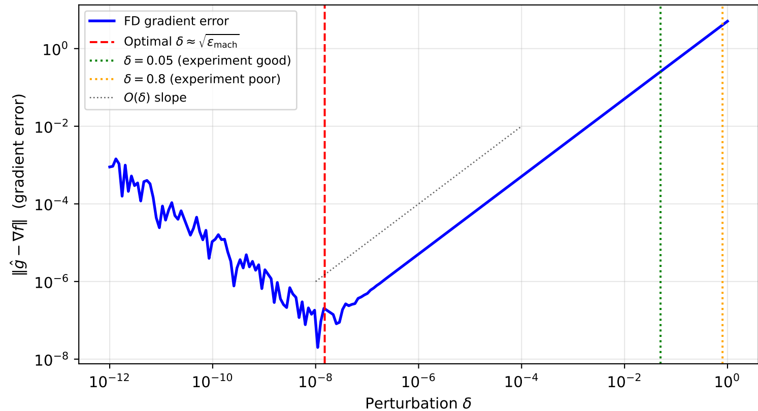
Q4: Finite-Difference Gradient Error vs Perturbation Size (Benchmark B, x = [0, 3]^T )
