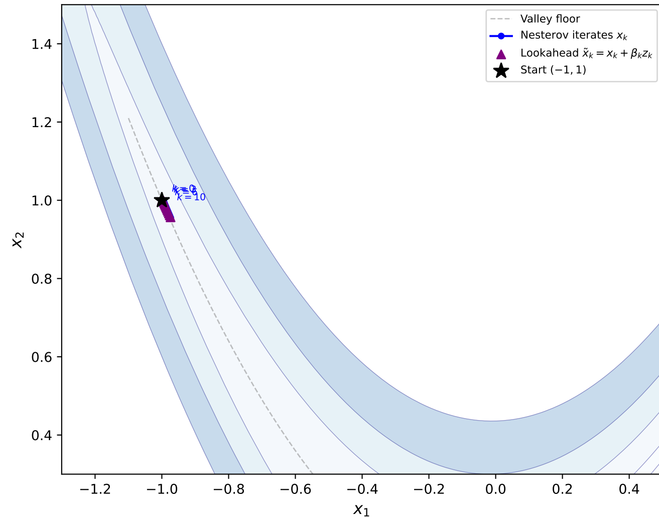
Nesterov Lookahead Extrapolation (First 15 iterations, \alpha = 0.0007 , \beta_{\max} = 0.90 )
