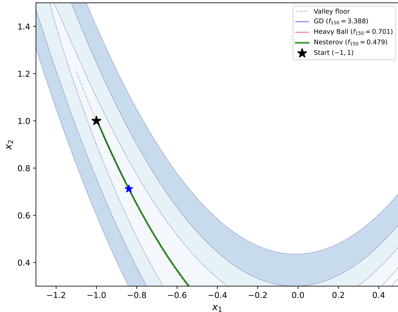
Trajectory Comparison at 150 Iterations: Nesterov vs Heavy Ball vs GD
