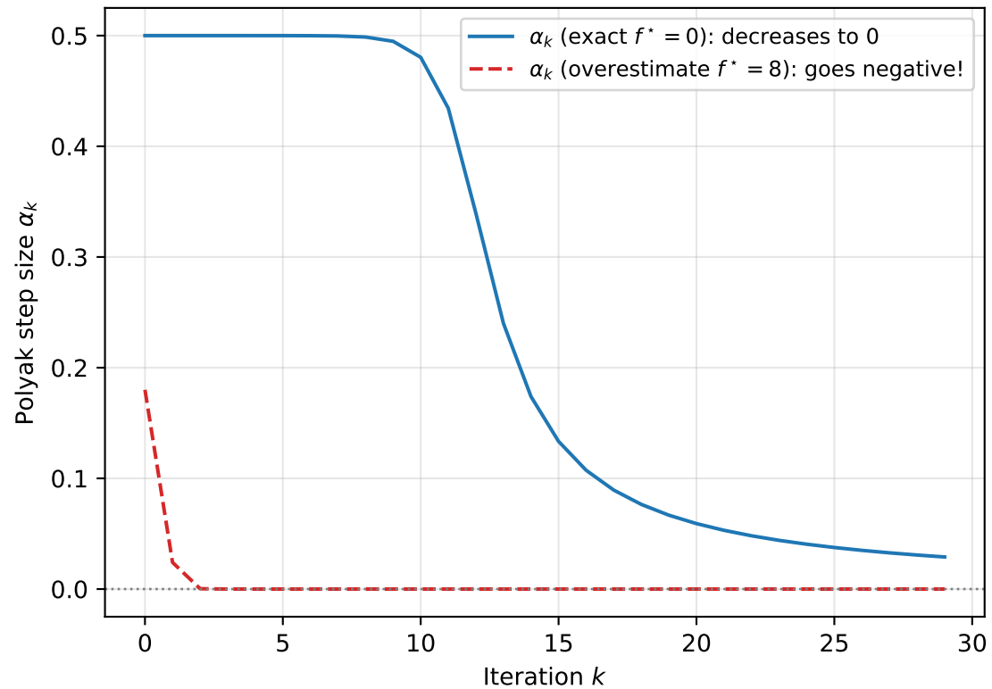
Step Size Dynamics: Exact vs Overestimated f^*
