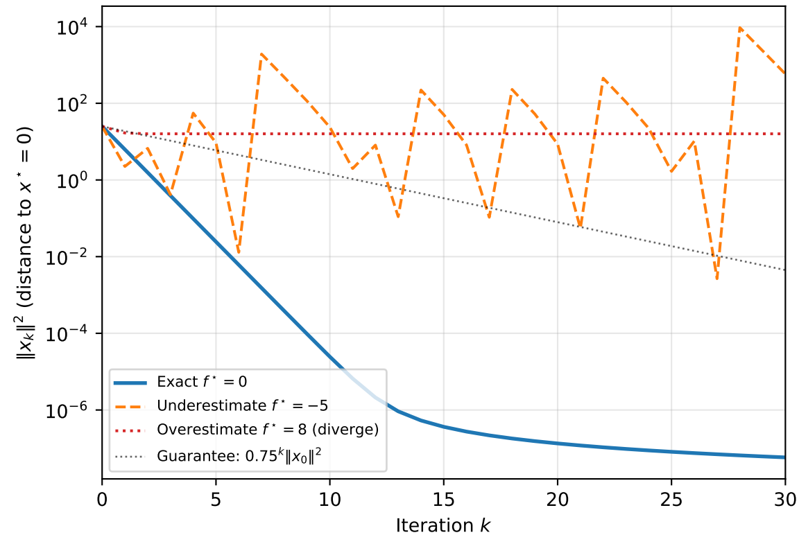
Polyak Step: Effect of f^* Specification
