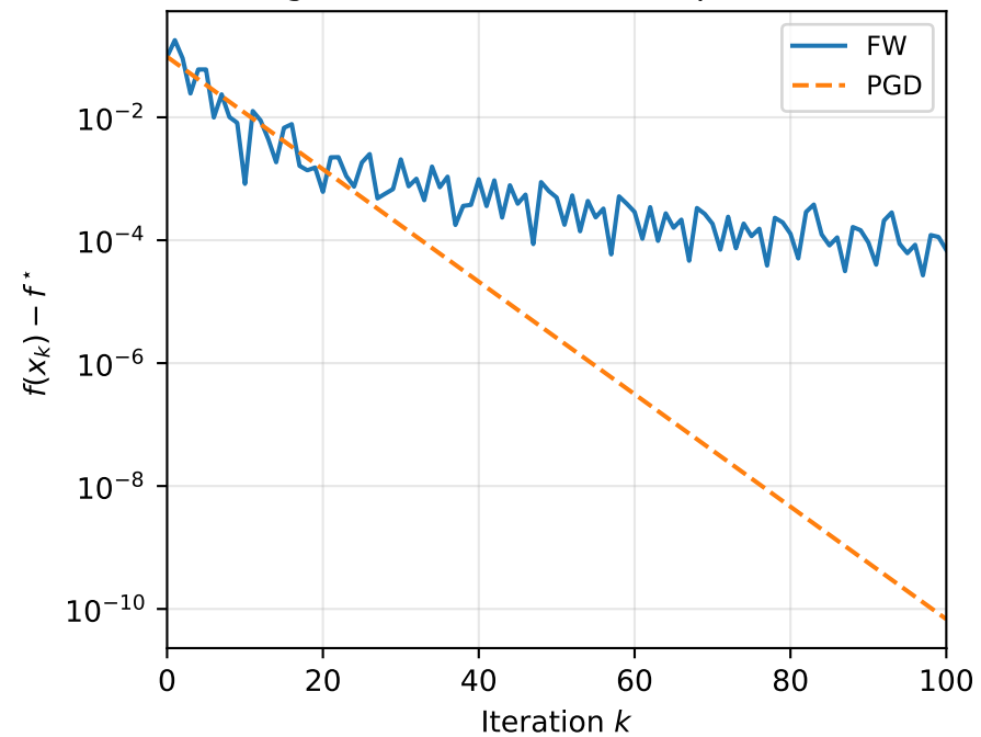
Convergence (FW slower but sparse iterates)
