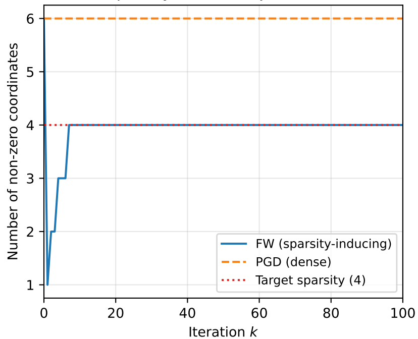
Sparsity: FW vs Projected GD
