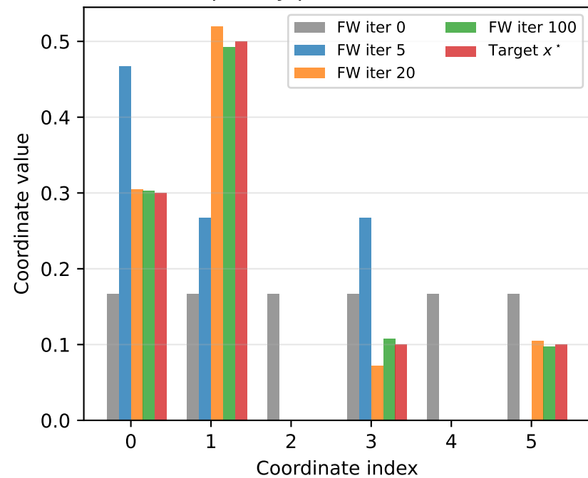
FW Iterates on the Simplex (sparsity pattern evolves)
