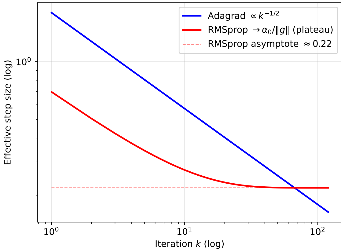
Log-log: Adagrad decay vs RMSprop plateau
