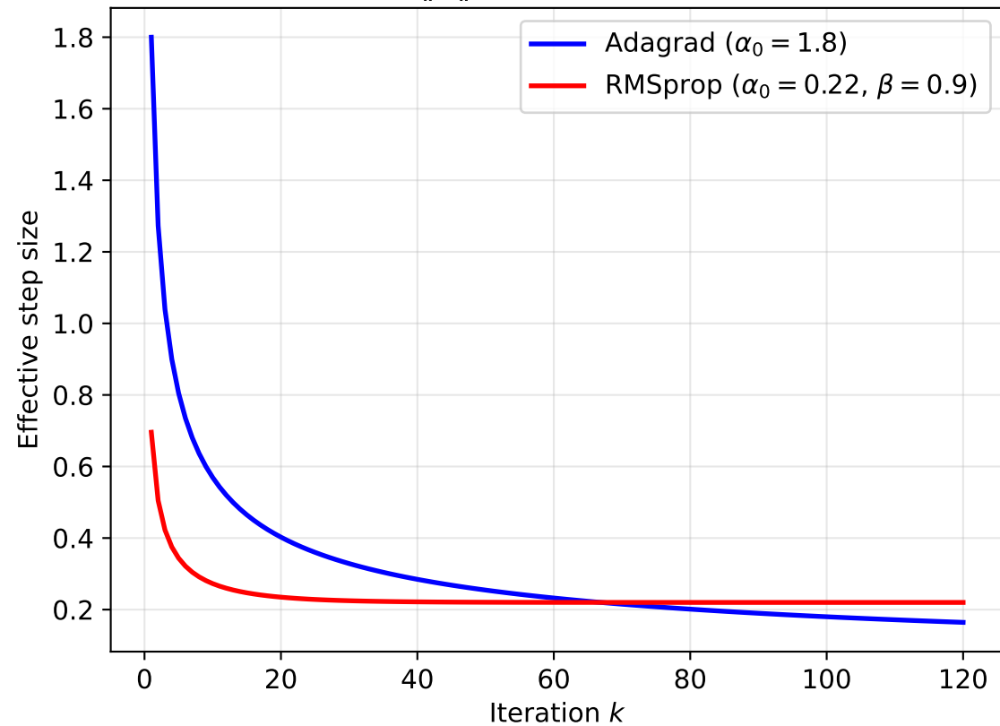
Theoretical Step Decay: Adagrad vs RMSprop (unit gradient \|g\| = 1 , Benchmark~A params)
