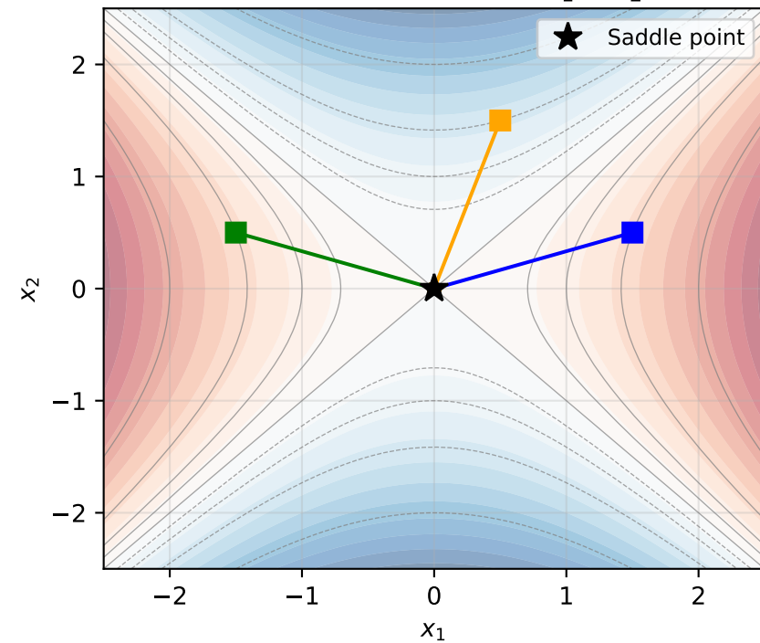
Newton on Saddle f = x_1^2 - x_2^2
