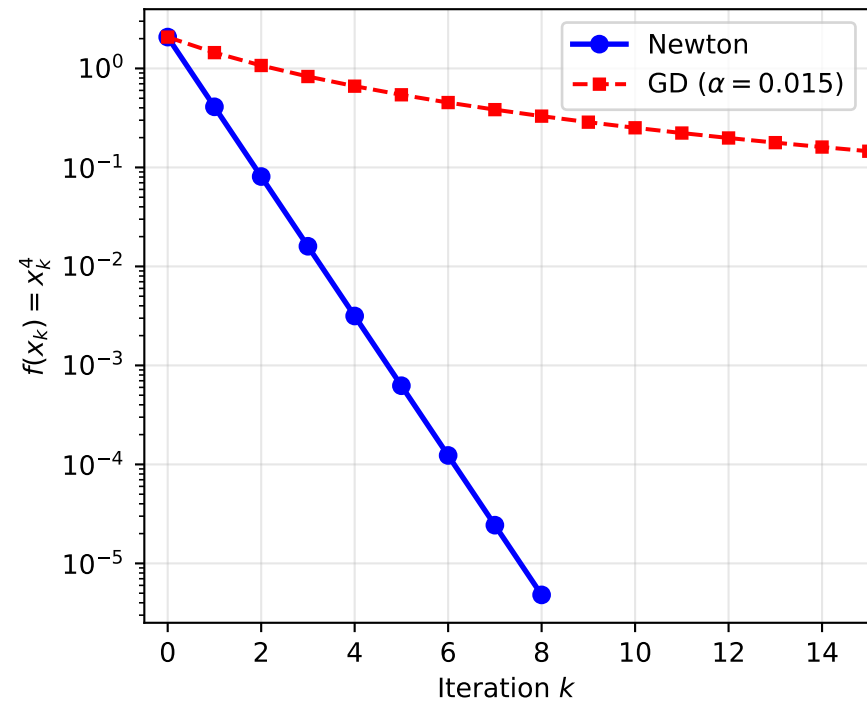
Newton vs GD on f(x) = x^4
