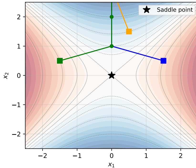
Safeguarded Newton (flip neg. eig.)
