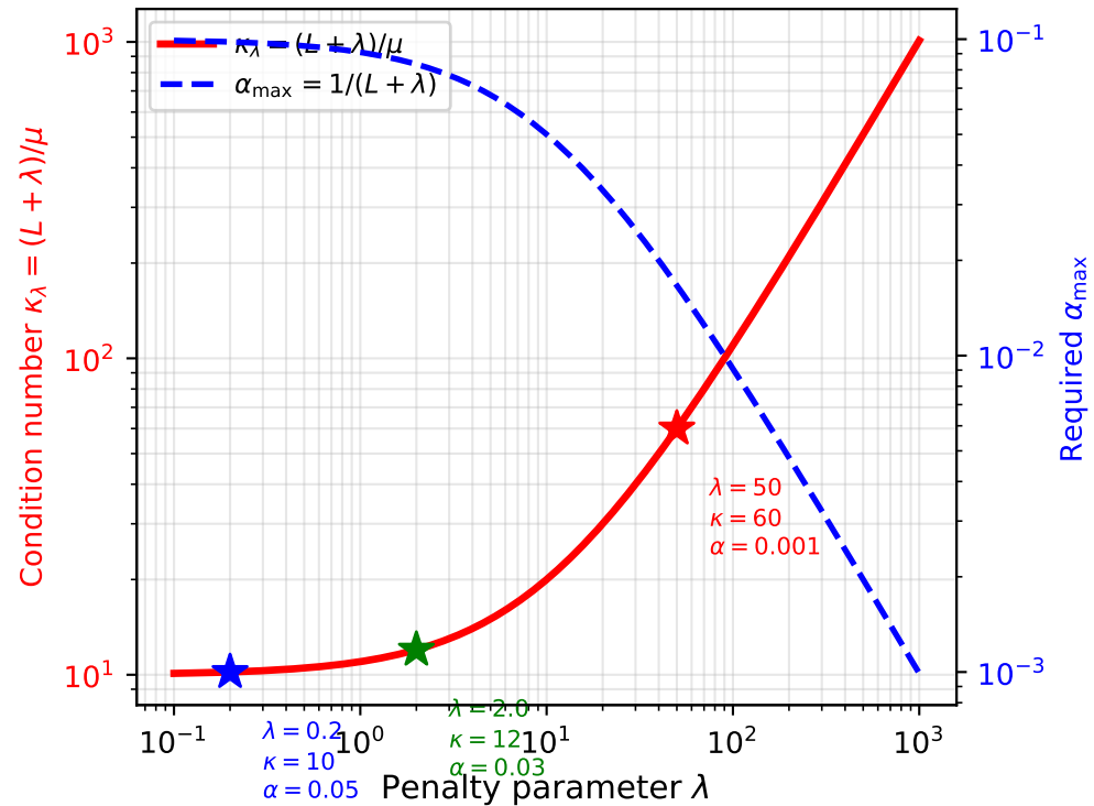
Ill-Conditioning from Large \lambda : \kappa_\lambda and Required Step Size
