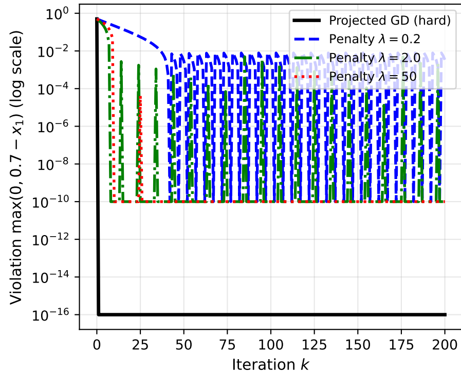
Active Constraint: Violation (PGD: zero from step 1)
