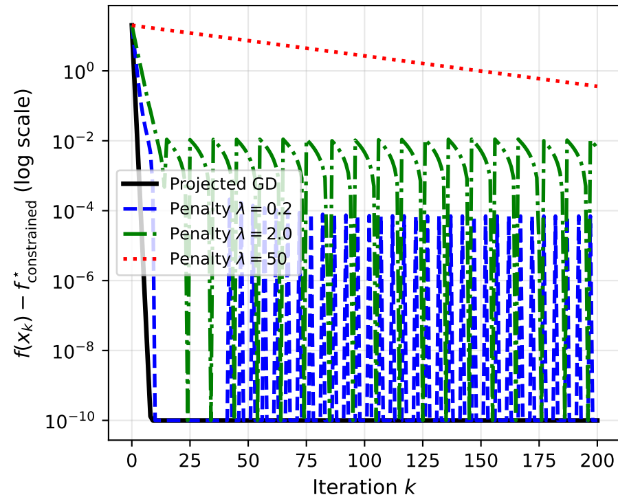
Active Constraint ( x_1 \geq 0.7 ) Objective Convergence
