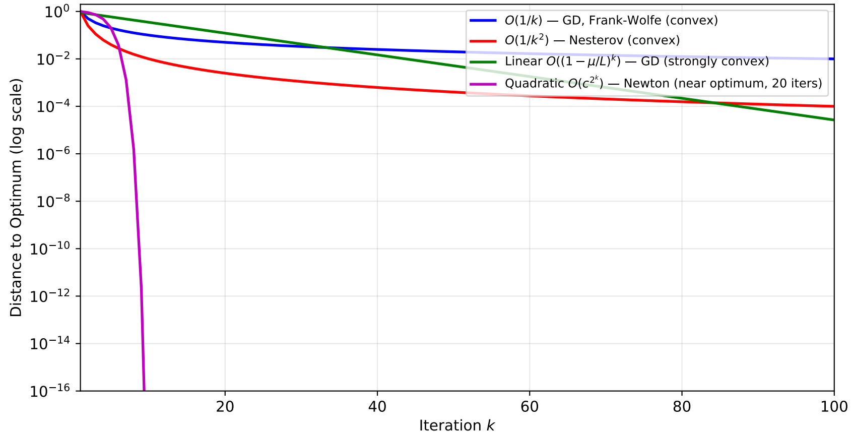
Theoretical Convergence Rates of Optimisation Algorithms
