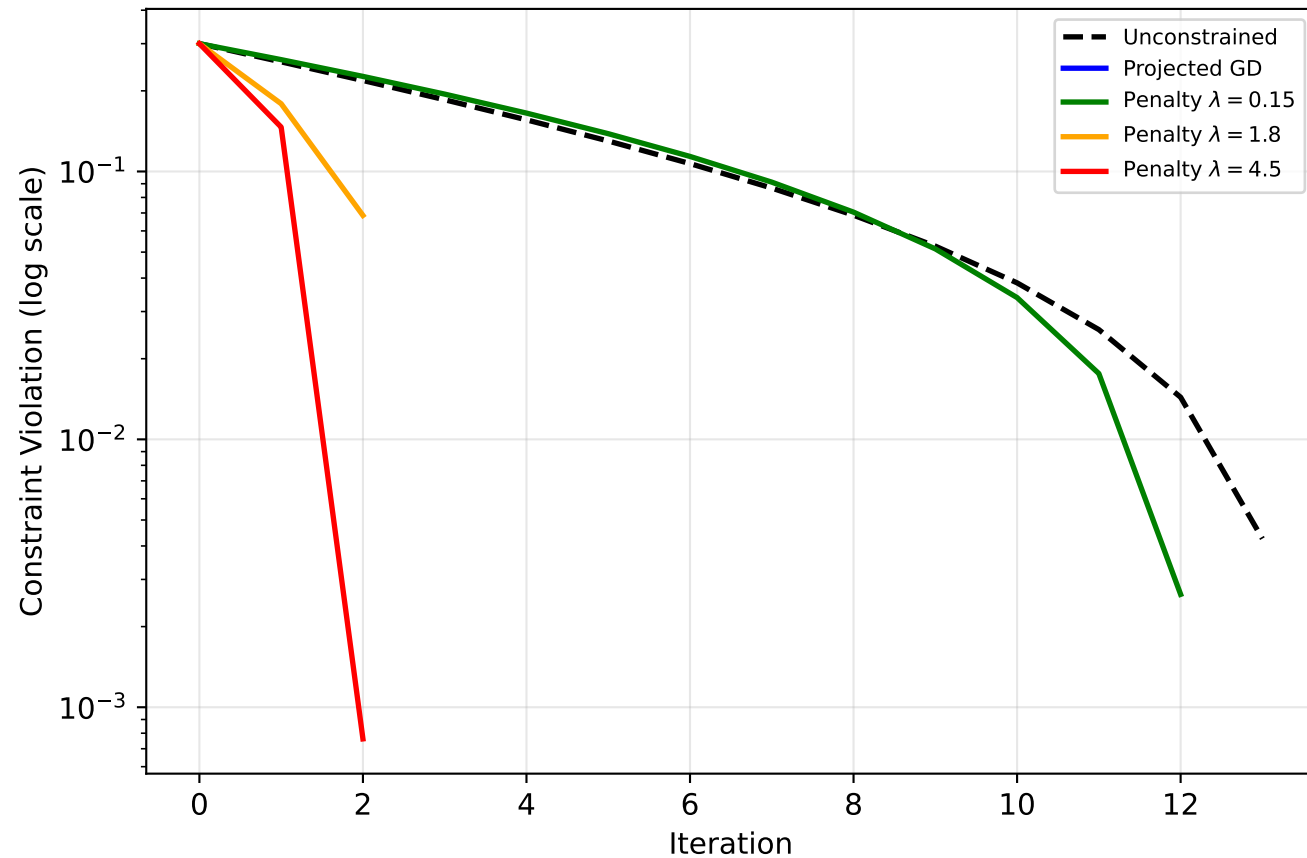
Q5: Constraint Violation \max(0, 0.5 - x_1)
