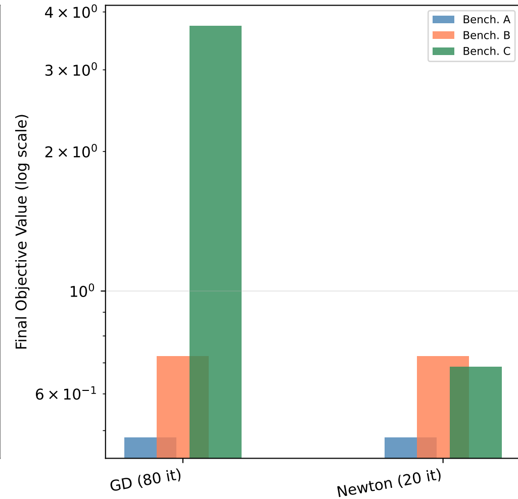
Q3: Newton's Method
