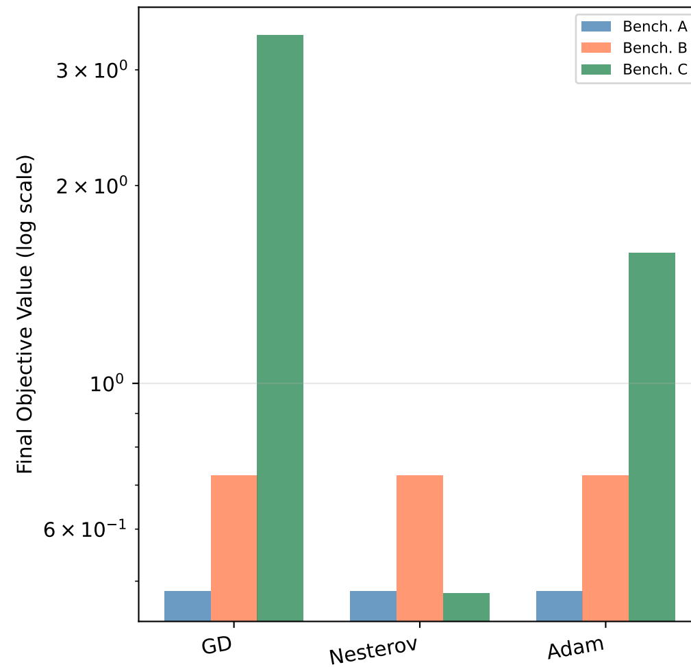
Q2: Momentum Methods
