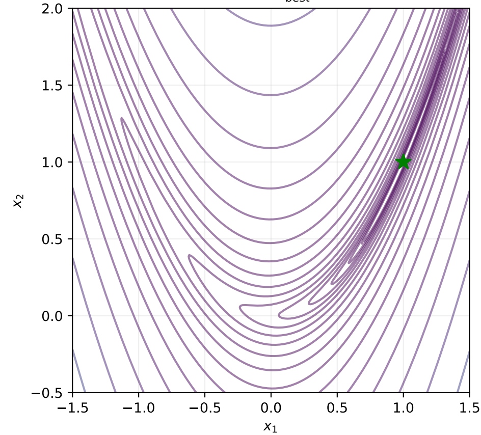
Iteration 159: f_{best} = 0.000
