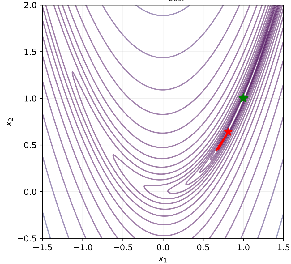
Iteration 99: f_{best} = 0.074
