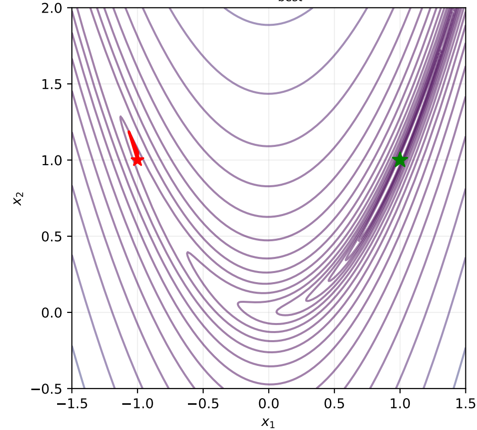
Iteration 159: f_{best} = 0.000
