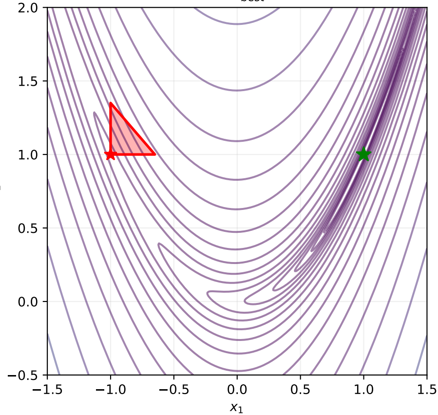
Iteration 49: f_{best} = 2.213
