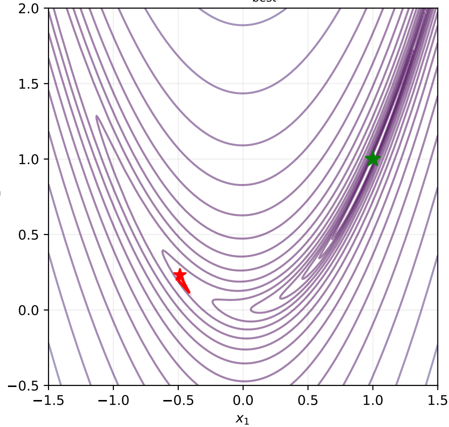
Iteration 49: f_{best} = 2.213
