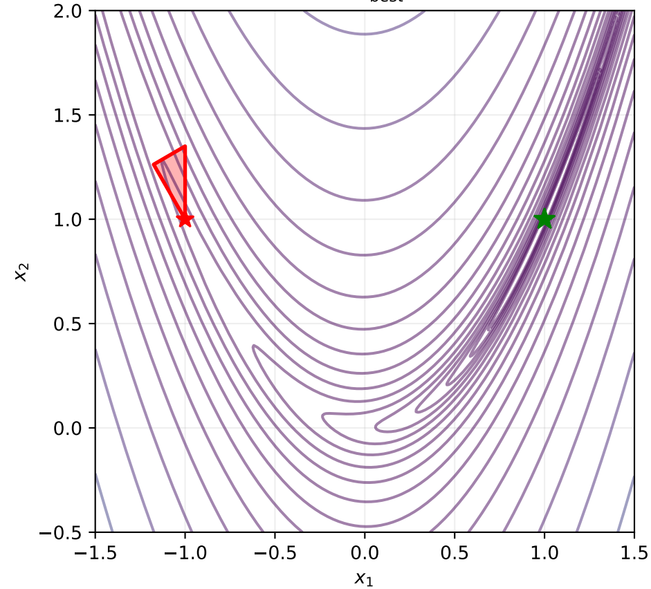
Iteration 99: f_{best} = 0.074
