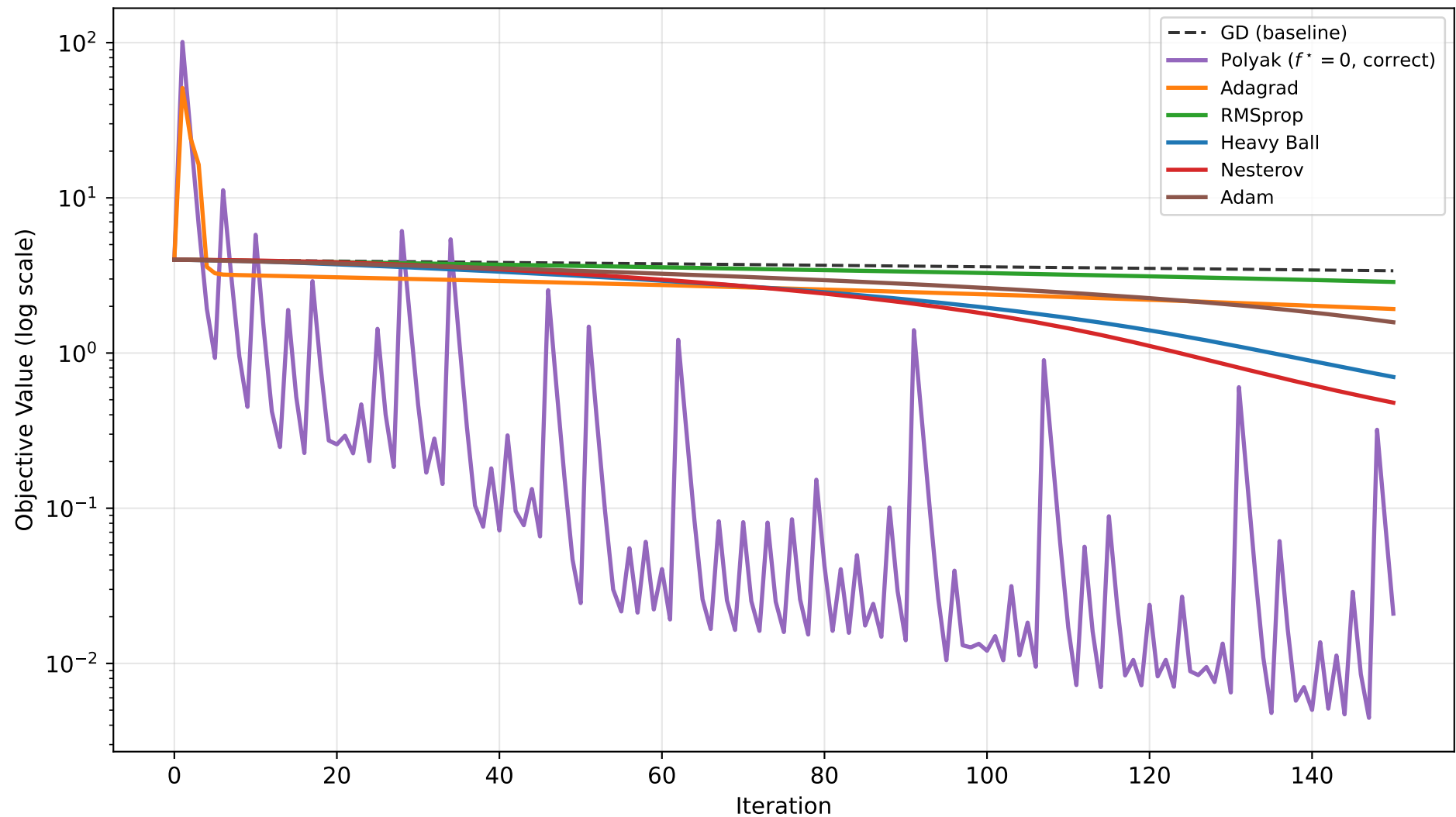
All First-Order Methods — Benchmark C (Rosenbrock), 150 iterations
