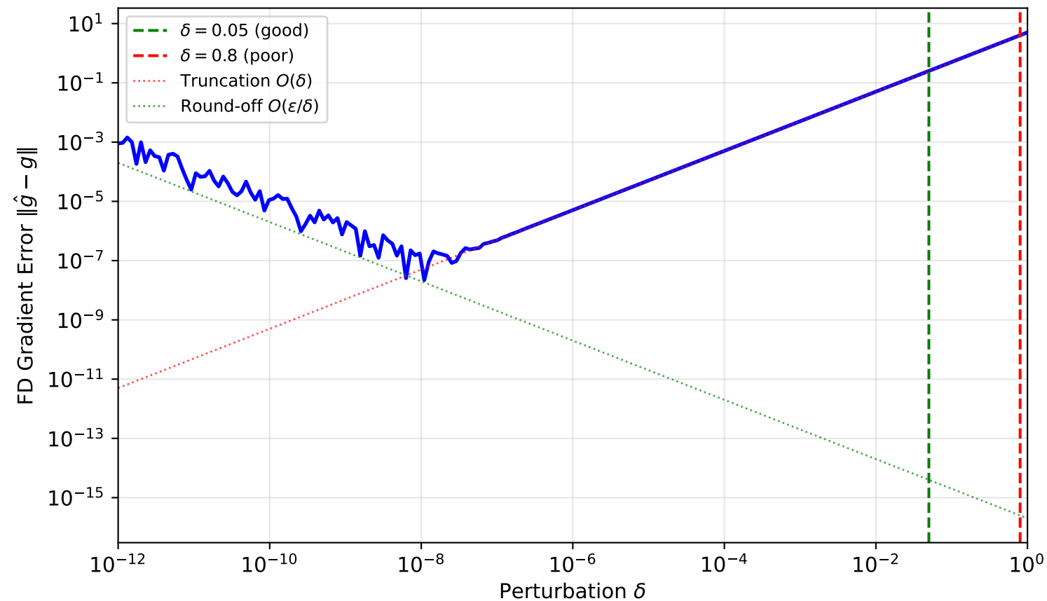
Q4: Finite Difference Gradient Error vs. Perturbation Size \delta
