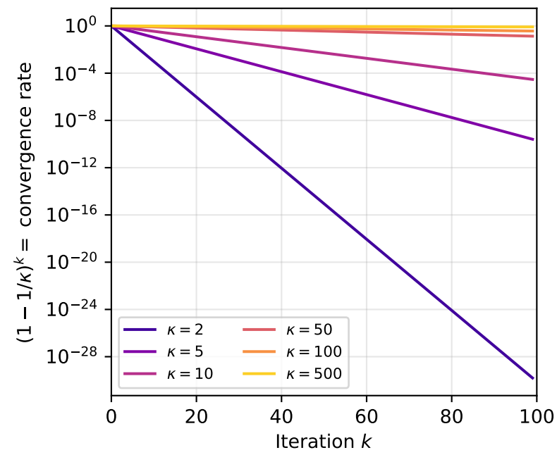
GD Convergence Rate vs \kappa
