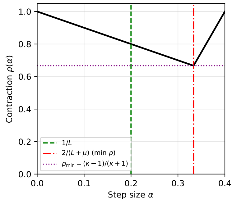
GD Contraction Factor
