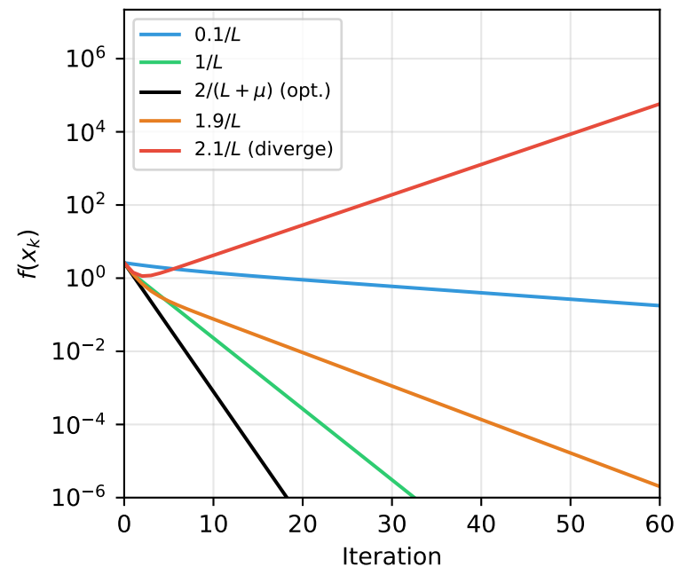
GD Step-Size Regimes ( \kappa = 5 )
