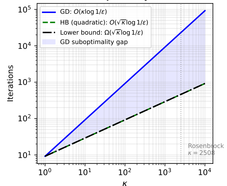
Lower Bounds: Optimality of Nesterov/HB
