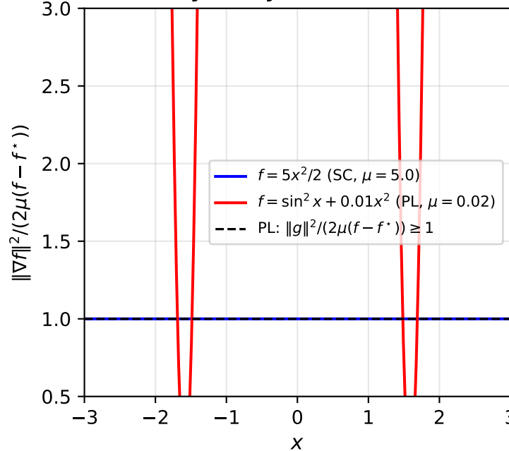
Polyak-Łojasiewicz Ratio
