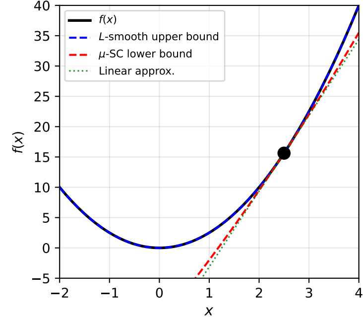
L-smooth and SC Function Bounds
