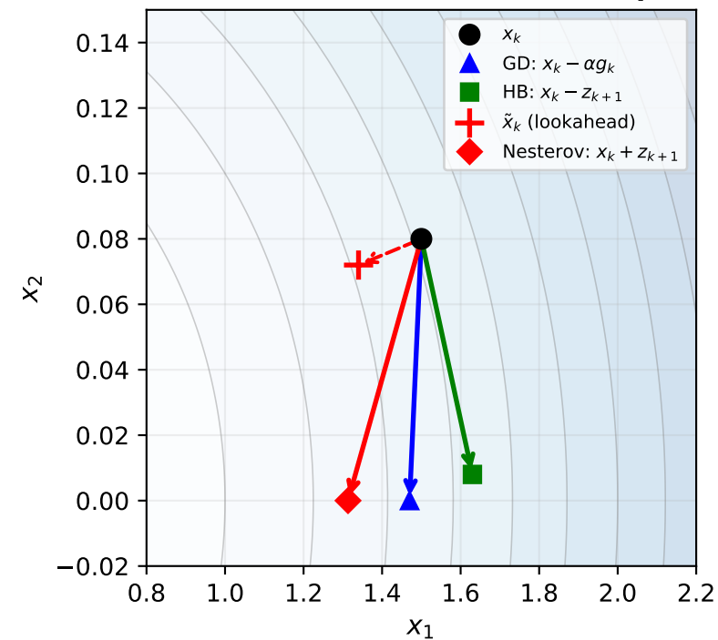
Nesterov Lookahead: One Step
