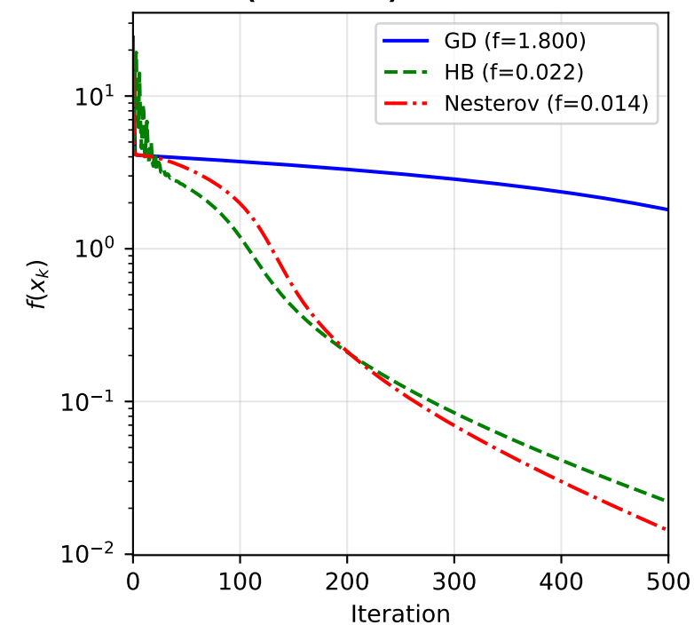
Rosenbrock (500 iters): GD vs HB vs Nesterov
