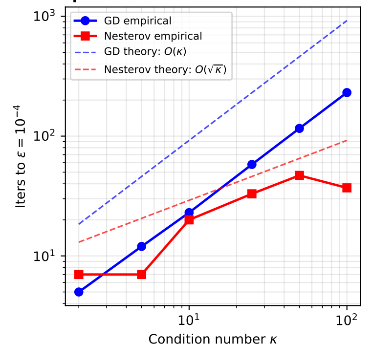
Empirical vs Theoretical Iteration Counts
