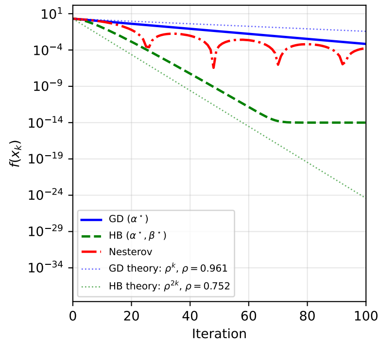
Quadratic ( \kappa = 50 ): Theory vs Empirical
