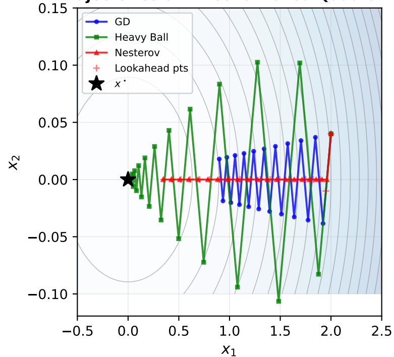
Trajectories on Ill-Conditioned Quadratic
