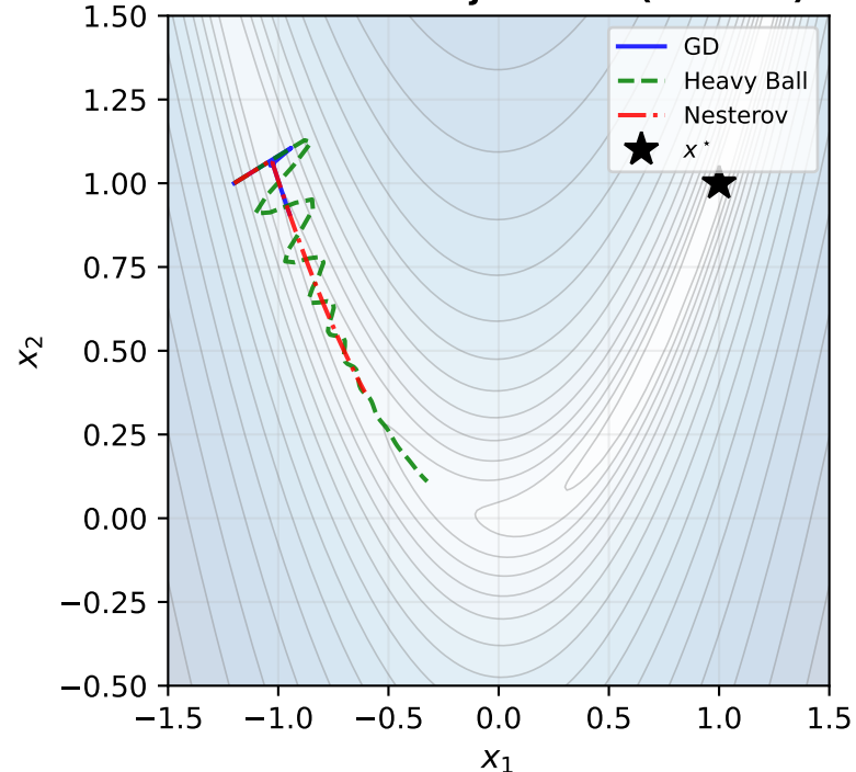
Rosenbrock Trajectories (80 iters)
