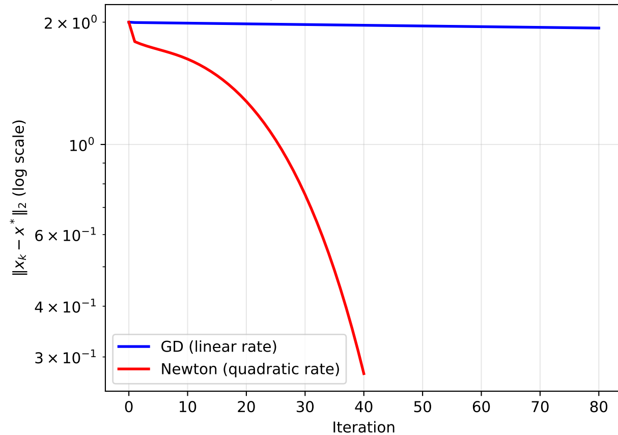
Q3: Distance to Optimum — Newton vs GD (Rosenbrock)
