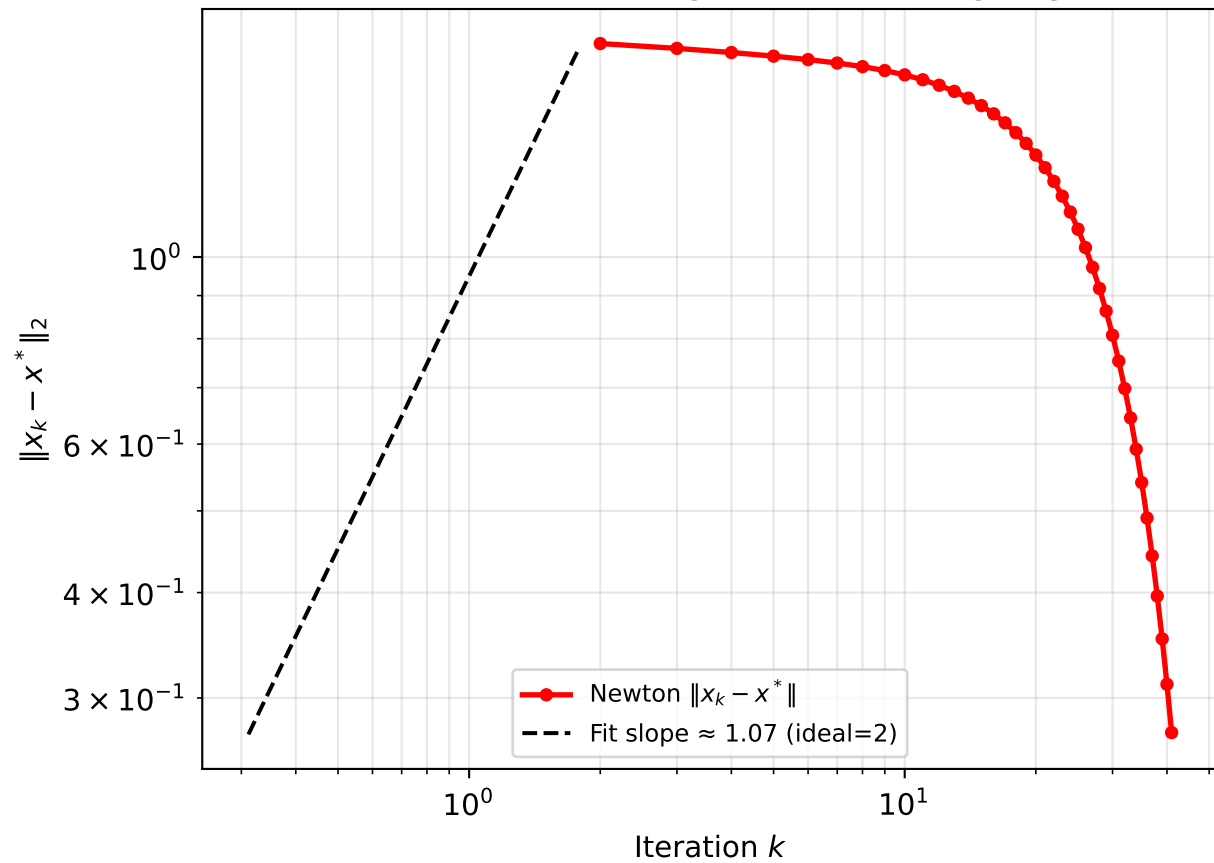
Q3: Newton Convergence Order (Log-Log)
