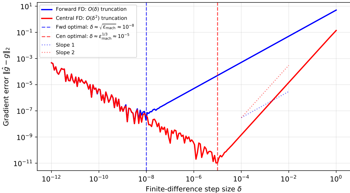
Q4: Finite-Difference Gradient Error vs Step Size (Benchmark B, evaluated at x = (0.5, 1.5) )
