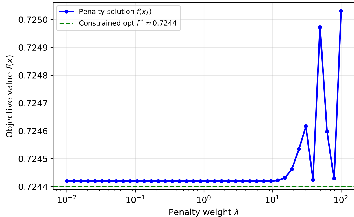
Q5: Objective Value vs Penalty Weight
