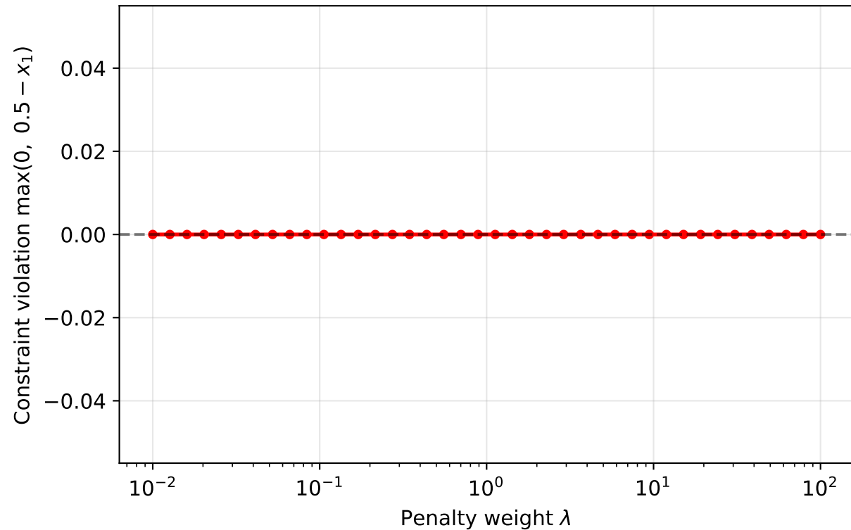
Q5: Constraint Violation vs Penalty Weight (after 200 iterations)
