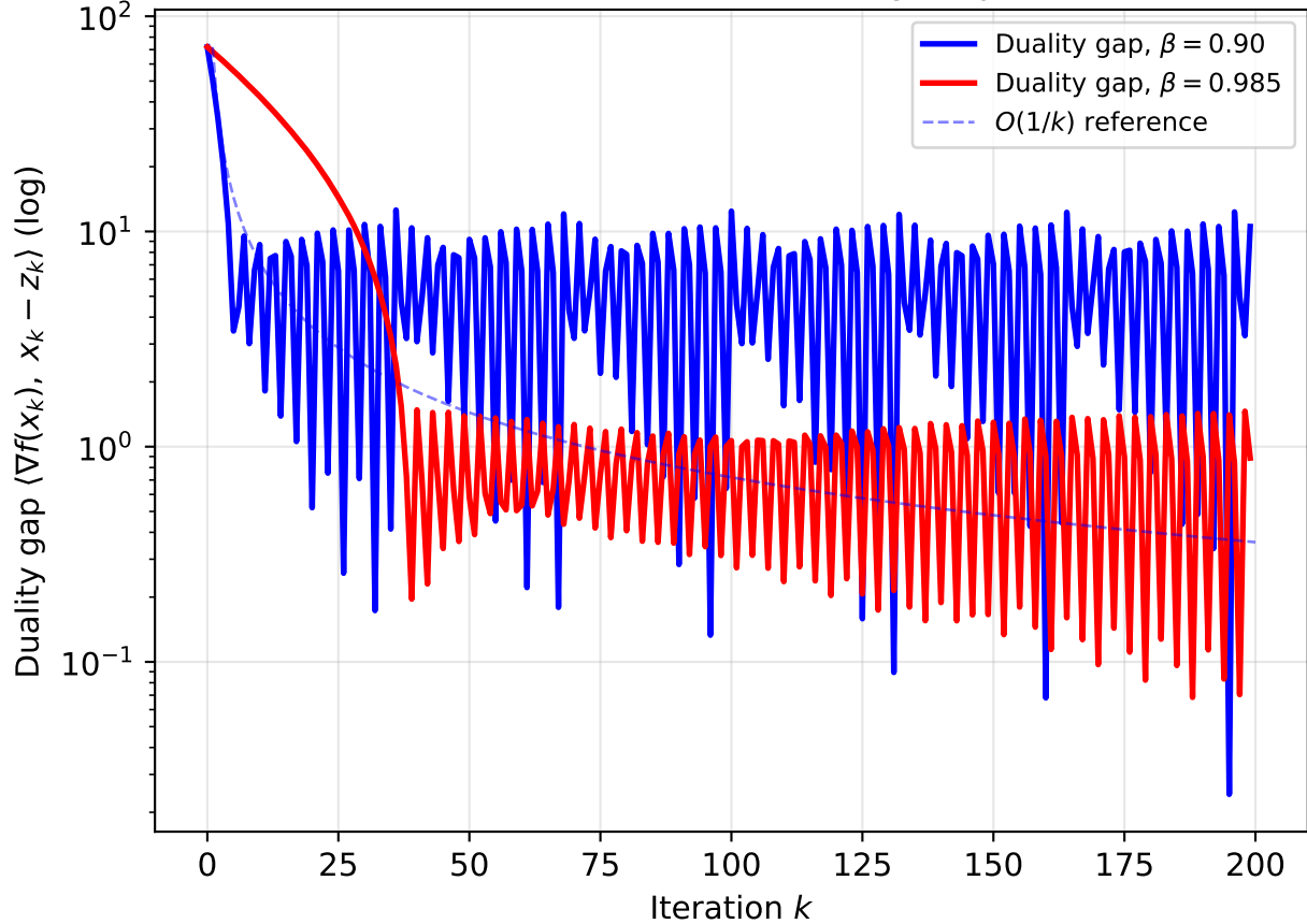
Q6: Frank-Wolfe Duality Gap
