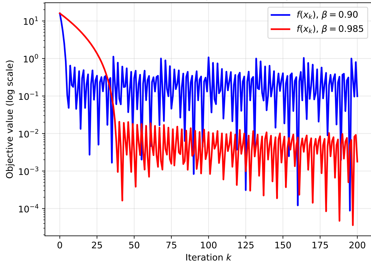
Q6: Frank-Wolfe Objective Convergence
