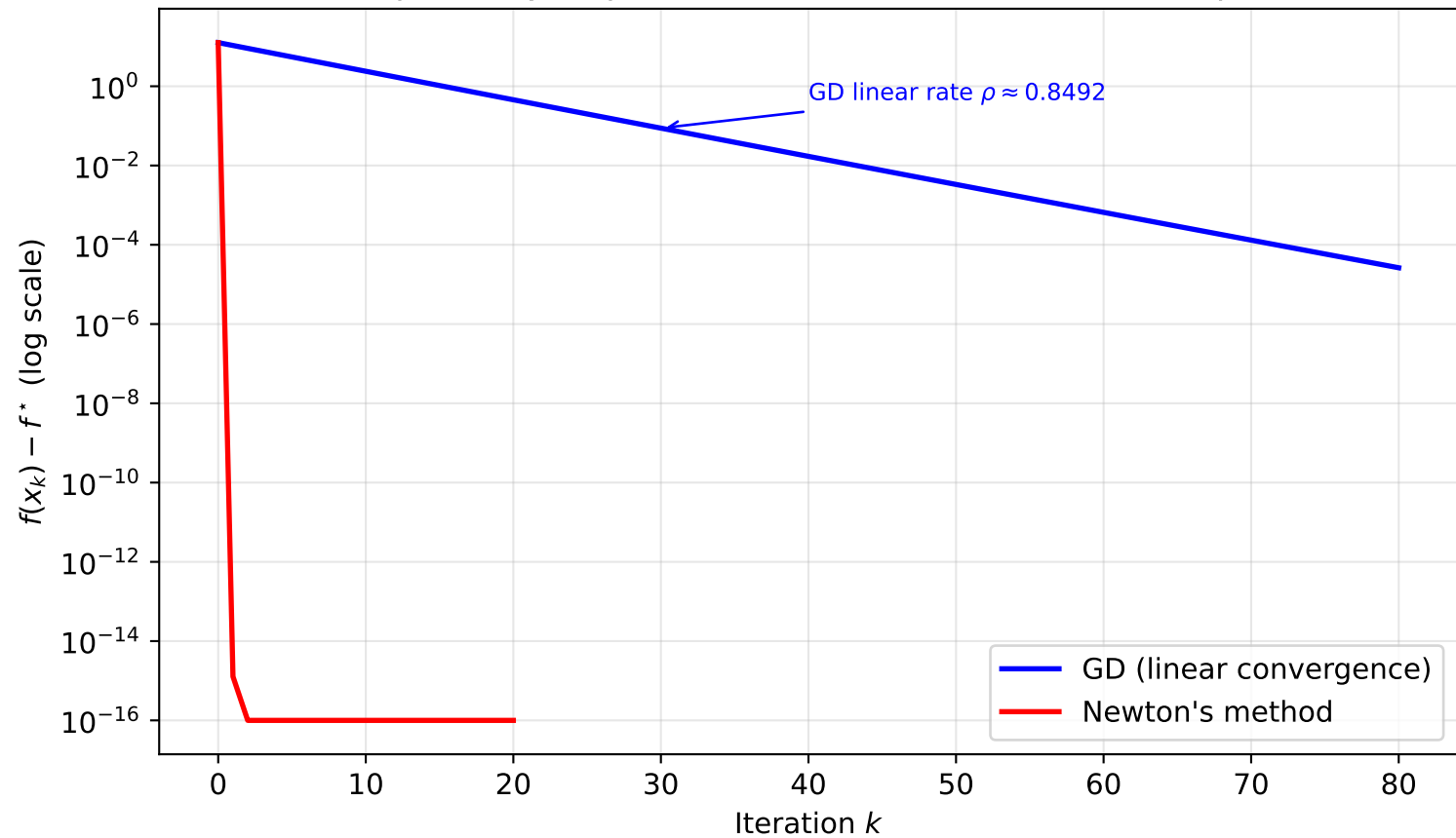
Q3: Suboptimality Gap — Newton vs GD (Benchmark A, quadratic)
