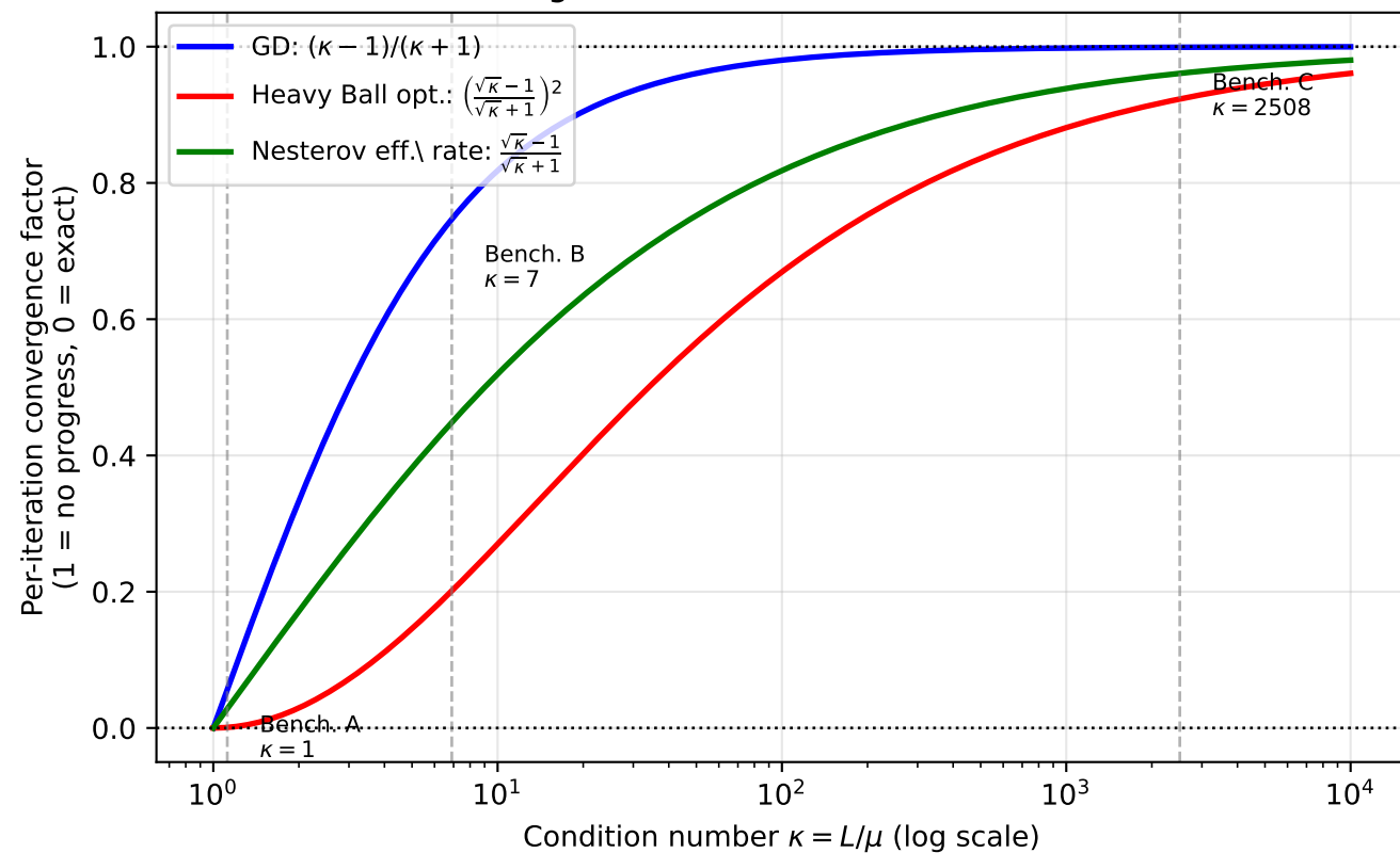
Convergence Factor vs Condition Number
