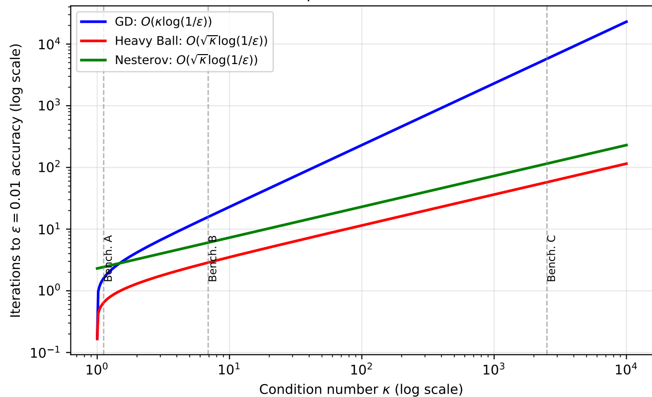
Iterations Required vs Condition Number
