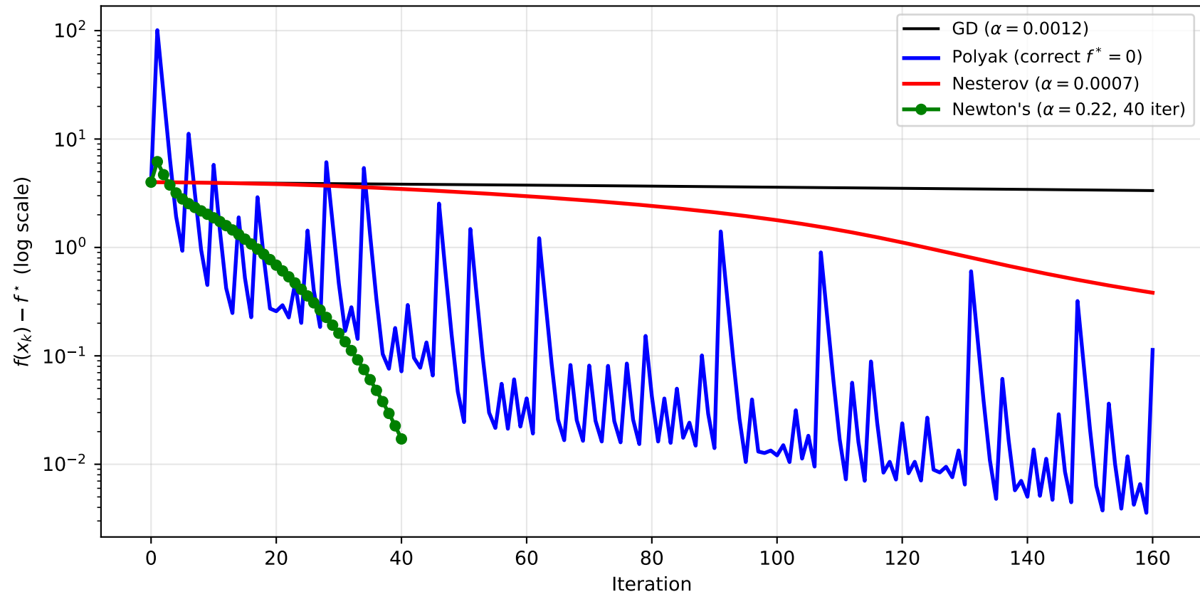
Benchmark C (Rosenbrock): Best Method per Category GD baseline vs Polyak (Q1) vs Nesterov (Q2) vs Newton (Q3)
