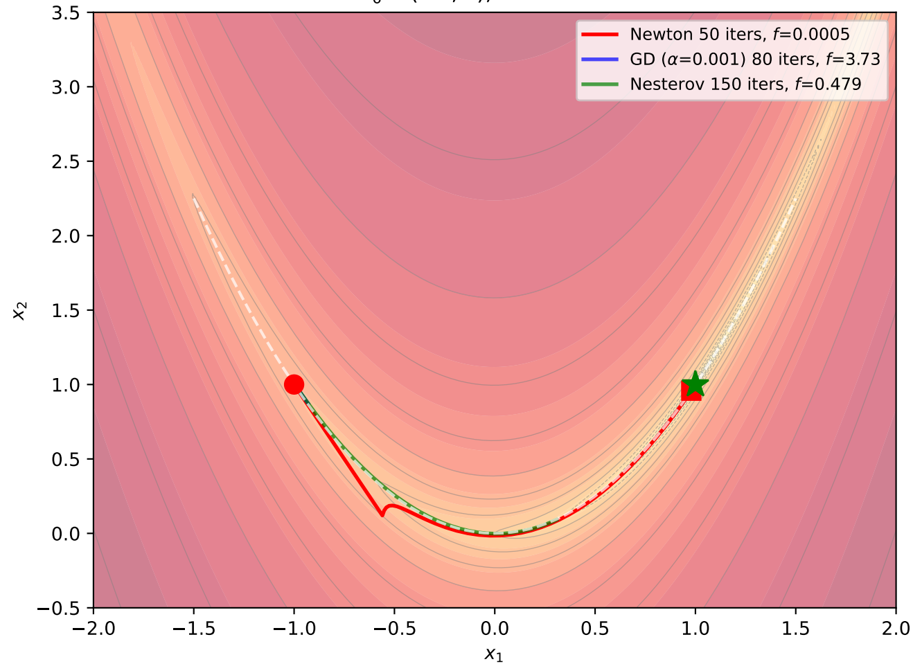
GD vs Newton vs Nesterov x_0 = (-1, 1) , Rosenbrock
