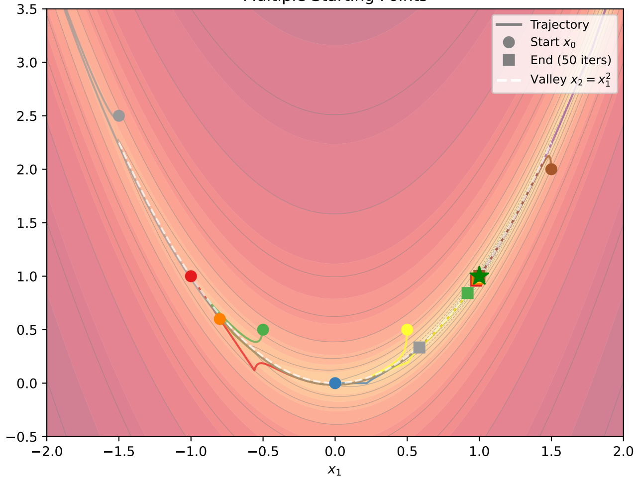
Newton ( \alpha = 0.22 , 50 iters) Multiple Starting Points
