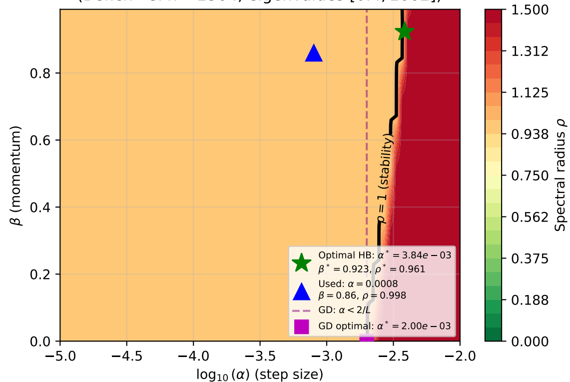
Heavy Ball Stability Map (Bench~C: \kappa \approx 2504 , eigenvalues [0.4, 1002] )
