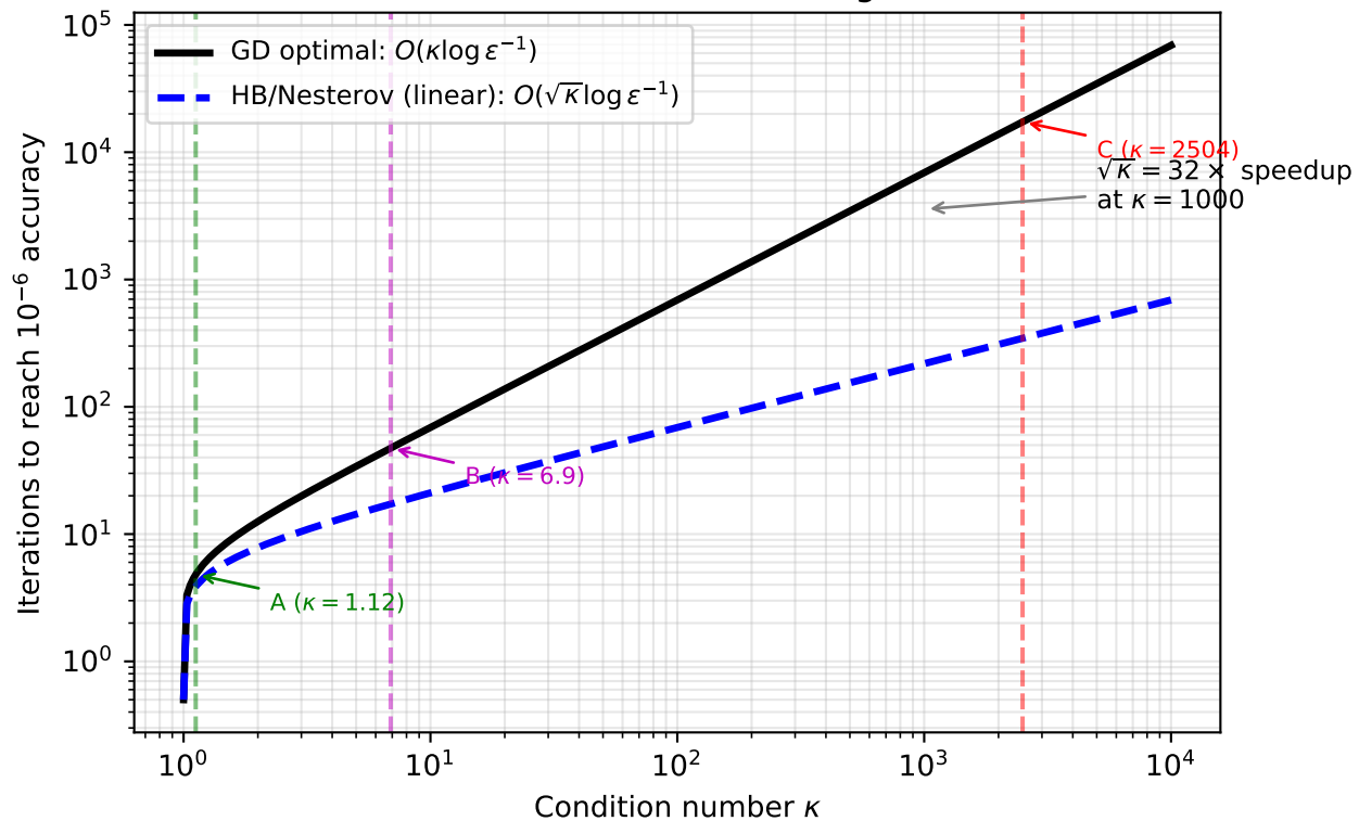
GD vs Optimal Heavy Ball Iteration Count Scaling
