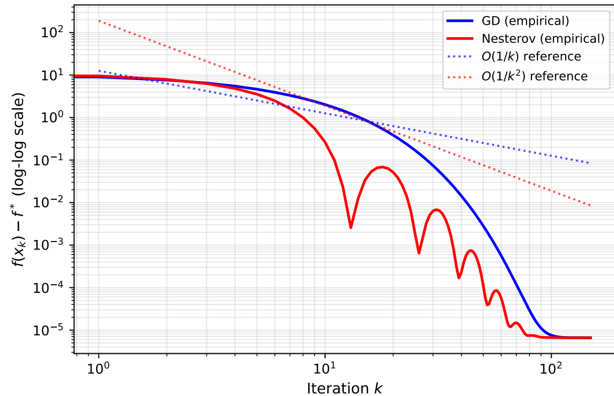
Benchmark A: Excess Objective vs Iteration
