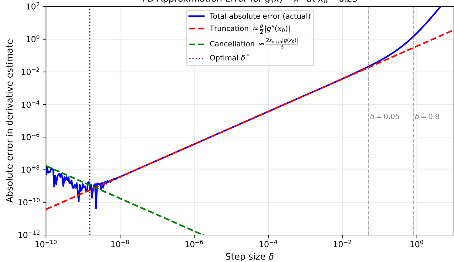
FD Approximation Error for g(x) = x^4 at x_0 = 0.25
