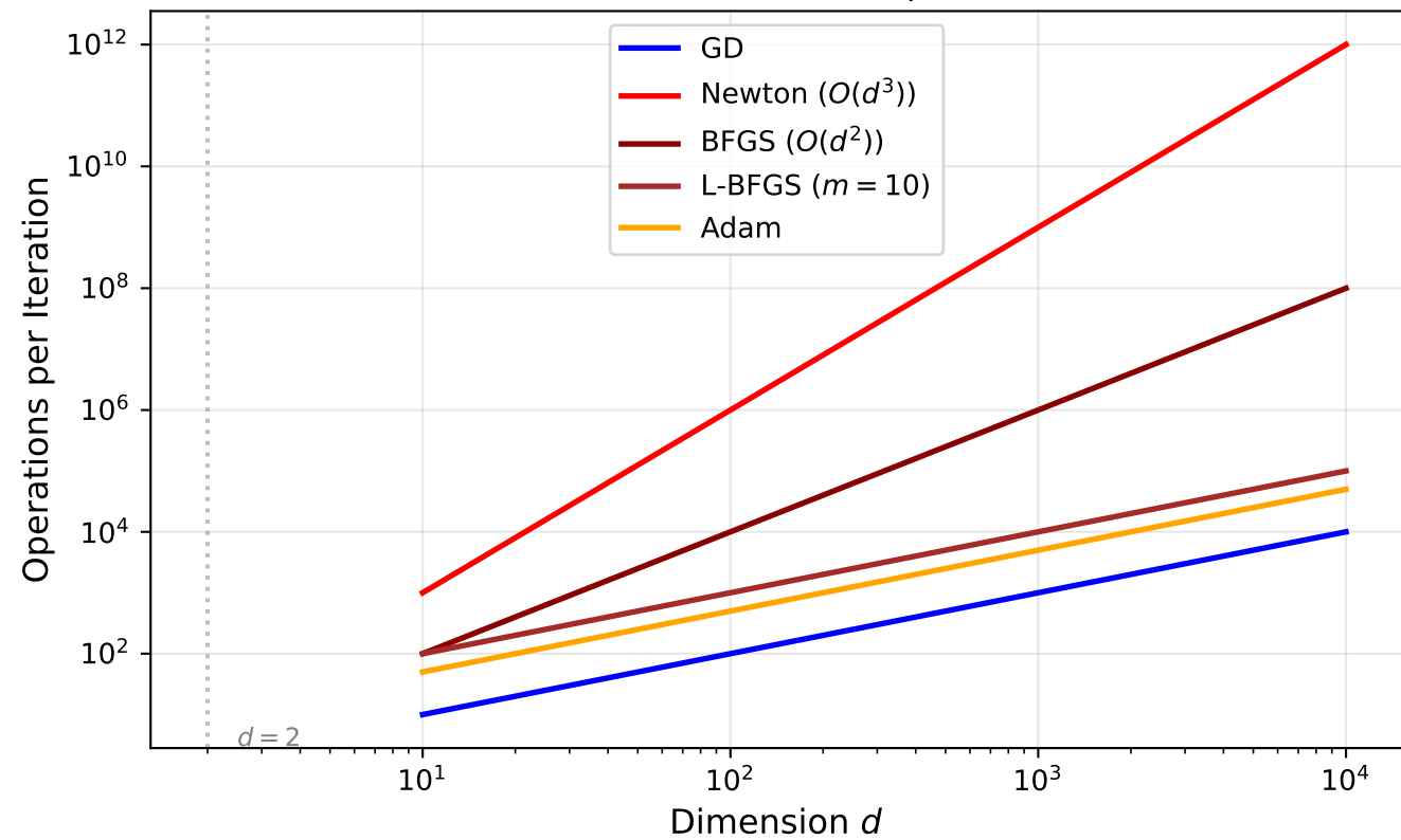
Gradient-Based Methods: Computational Cost
