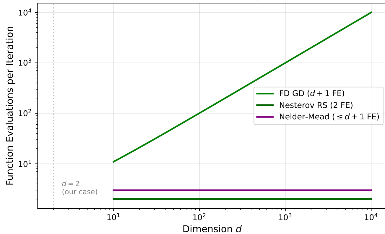
Derivative-Free Methods: Cost per Iteration
