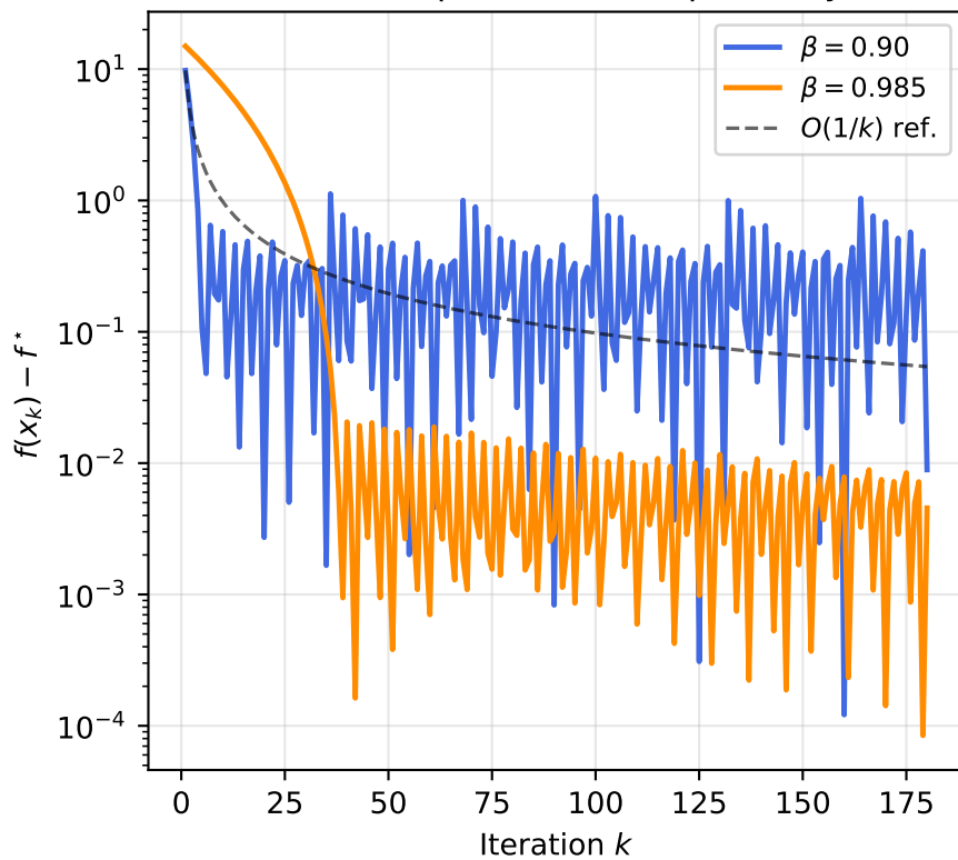
Interior Optimum: Suboptimality
