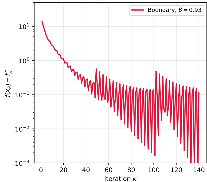
Boundary Optimum: Persistent Gap
