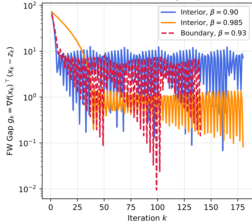
Frank-Wolfe Duality Gap
