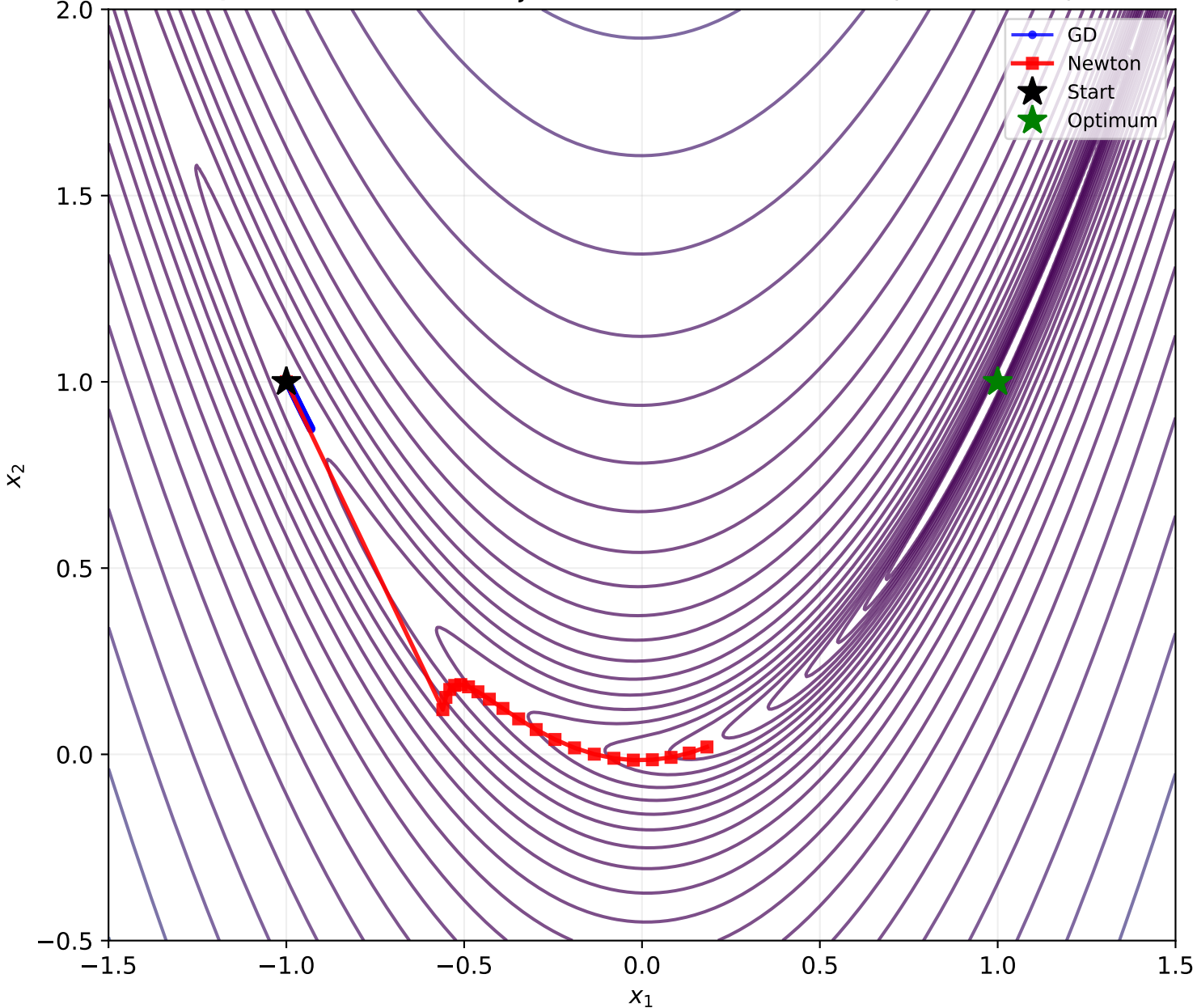
Q3: Newton vs GD Trajectories — Benchmark C (Rosenbrock)
