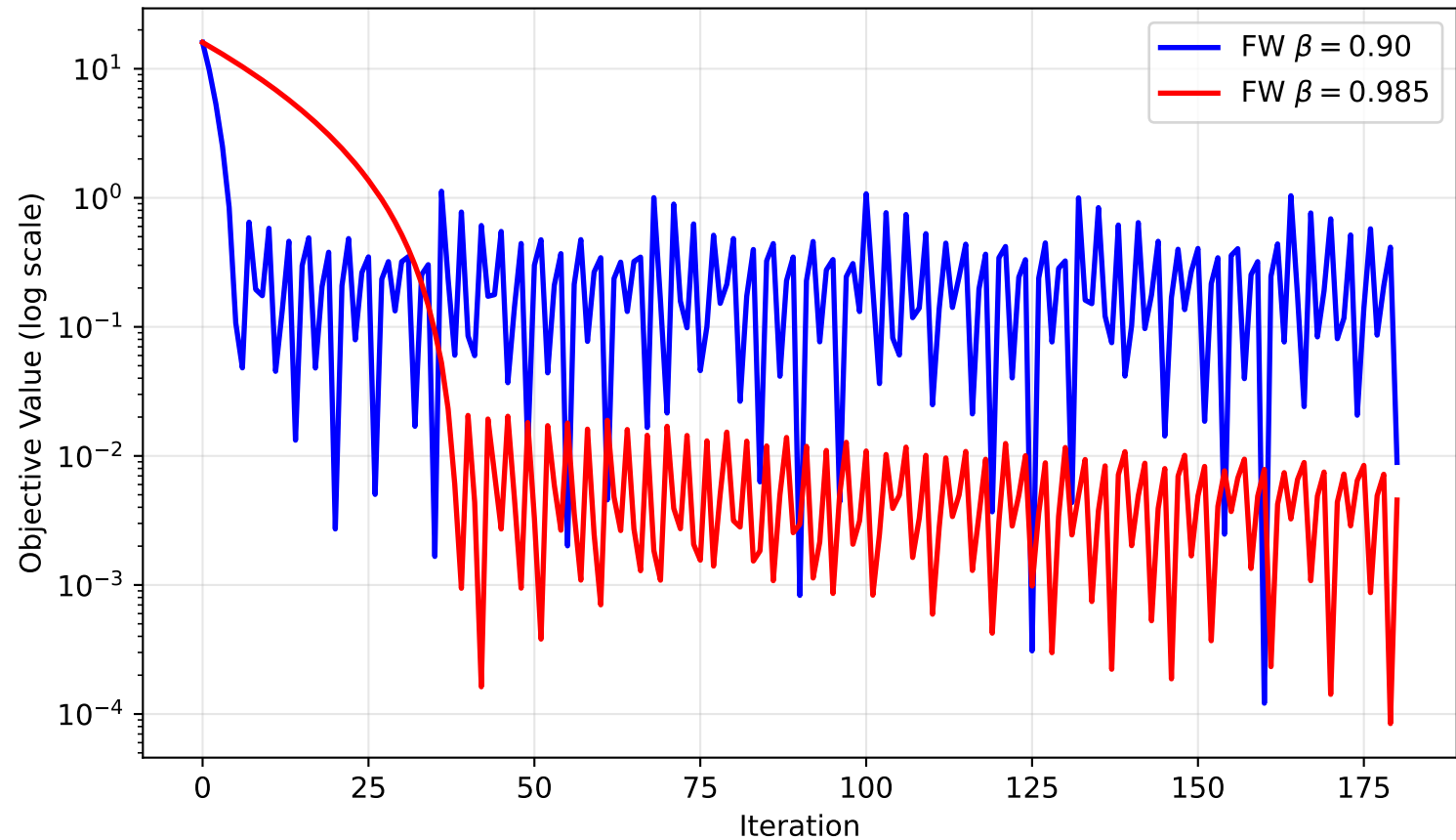
Q6-II: Frank-Wolfe Convergence — Interior Optimum
