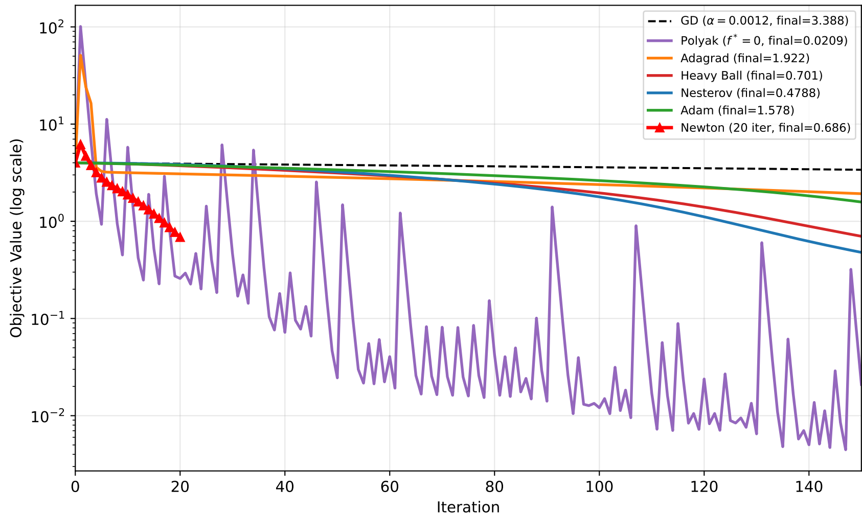
Benchmark C (Rosenbrock): All Methods Compared Q1 methods: 150 iter; Newton (Q3): 20 iter; f^* = 0
