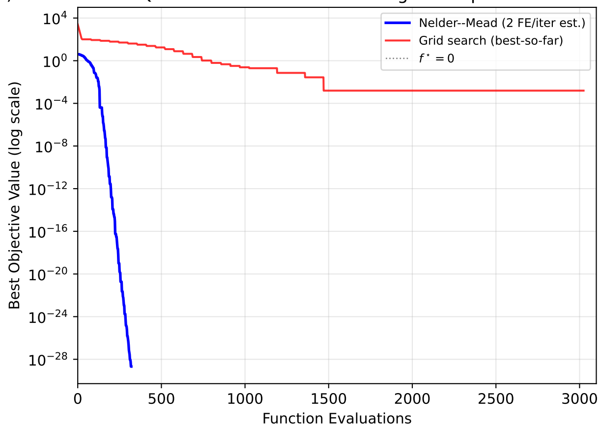
Q4B: Function Evaluation Budget Comparison
