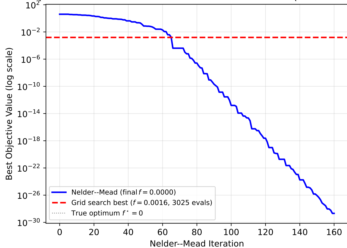
Q4B: Nelder--Mead vs Grid Search — Benchmark C (Rosenbrock)
