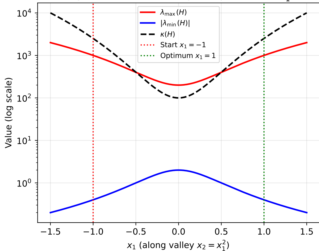
Eigenvalues and \kappa along valley floor x_2 = x_1^2
