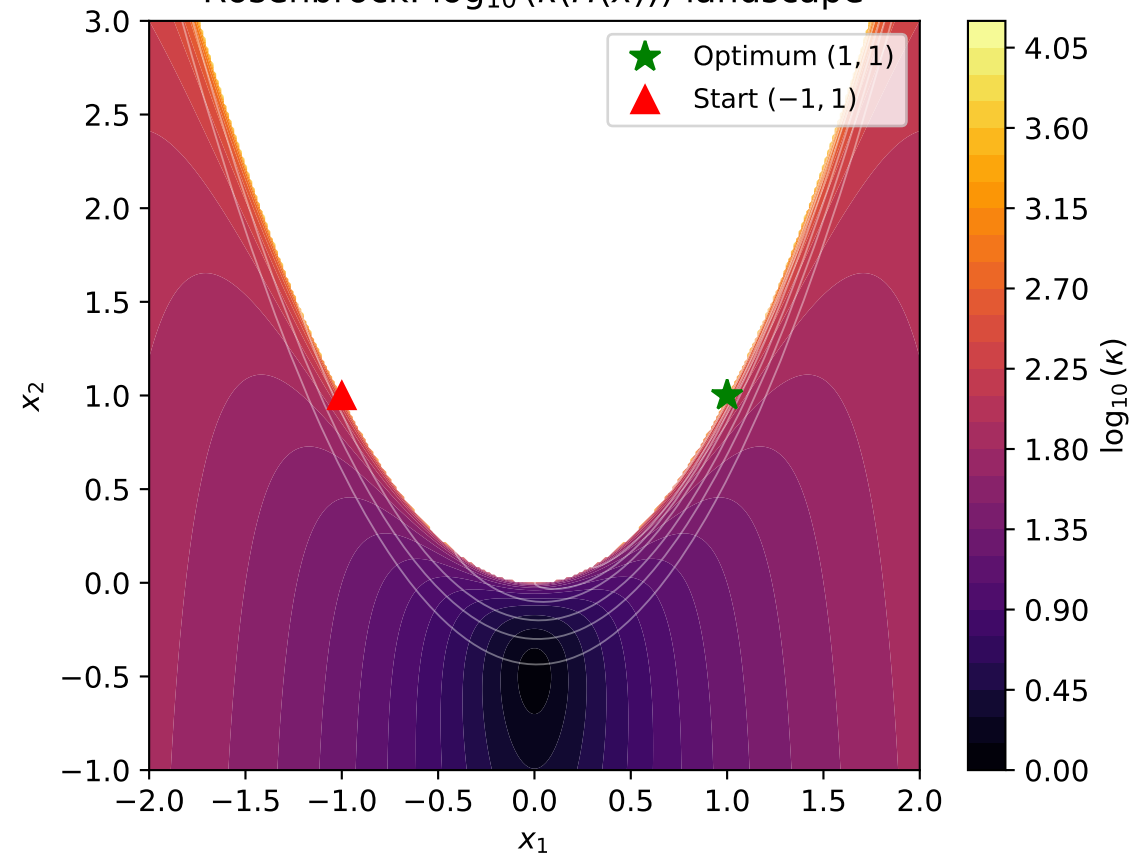
Rosenbrock: \log_{10}(\kappa(H(x))) landscape
