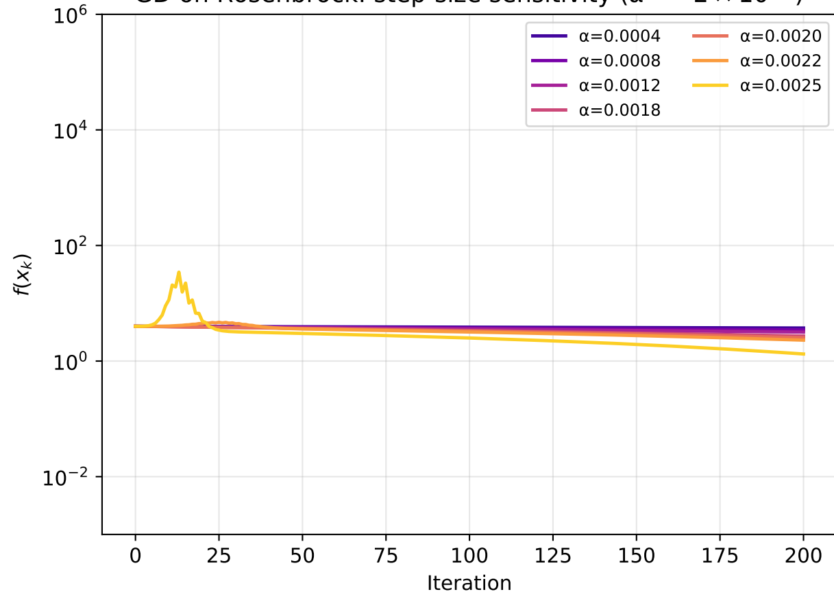
GD on Rosenbrock: step-size sensitivity ( \alpha^* \approx 2 \times 10^{-3} )
