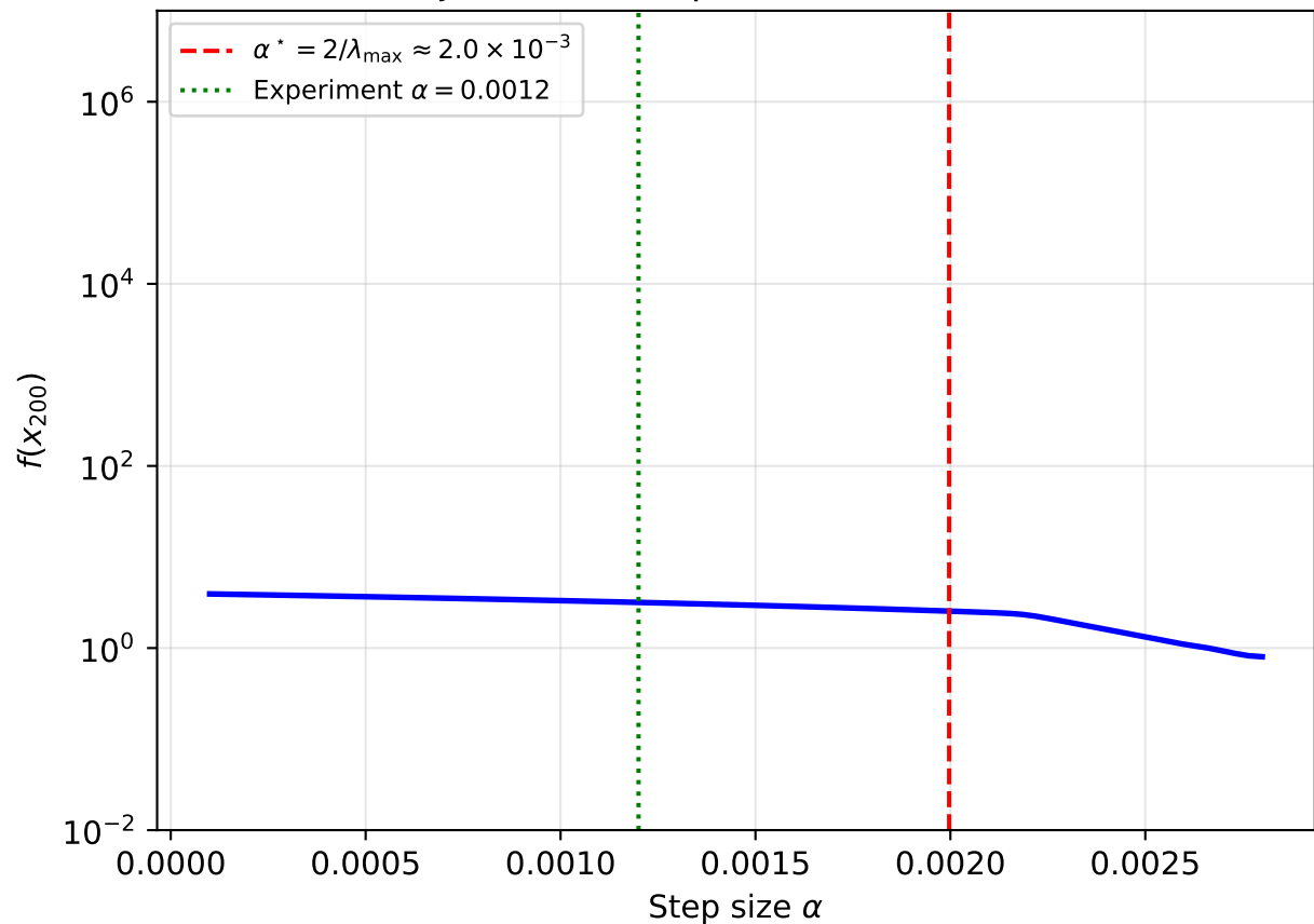
Final objective vs step size after 200 iterations
