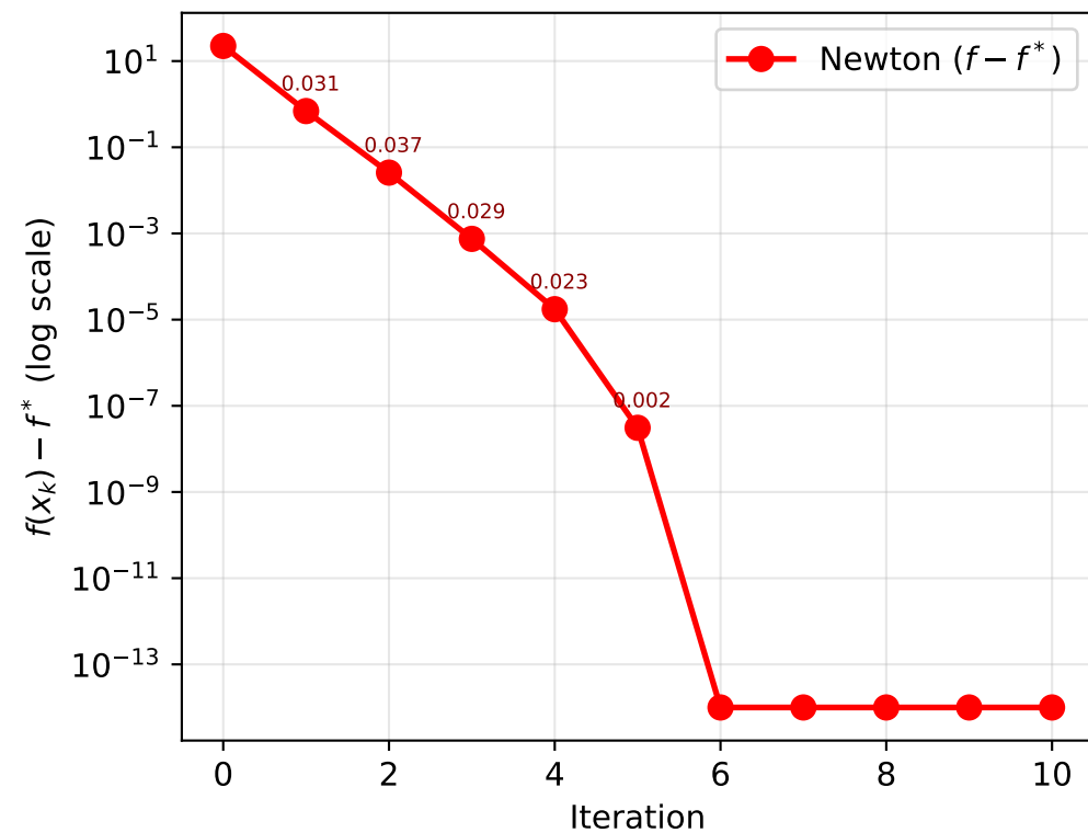
Newton Super-Linear Convergence Benchmark B
