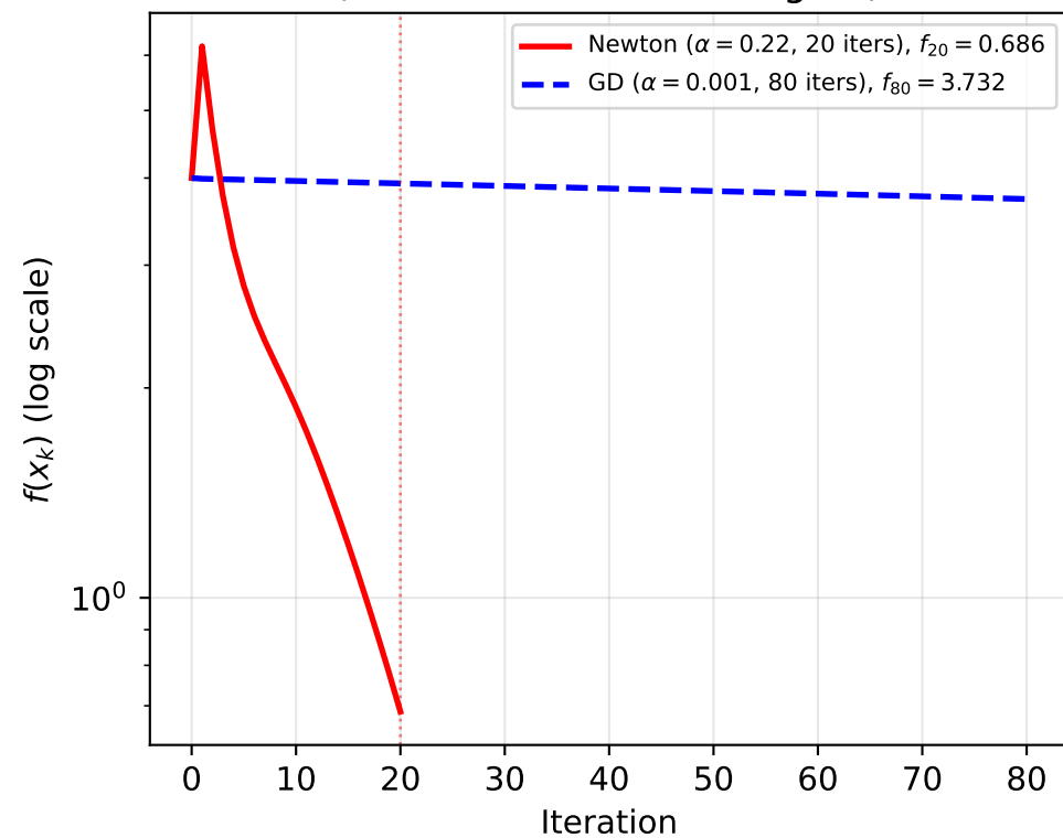
Newton vs GD on Rosenbrock (Different iteration budgets)
