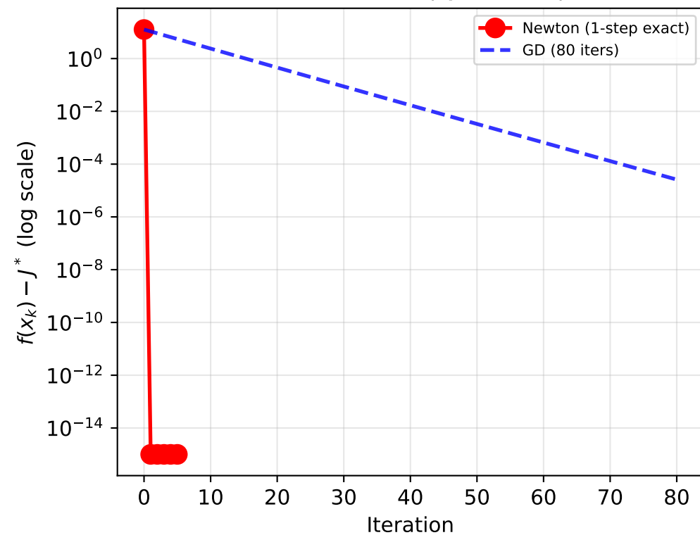
Newton One-Step Convergence Benchmark A (Quadratic)
