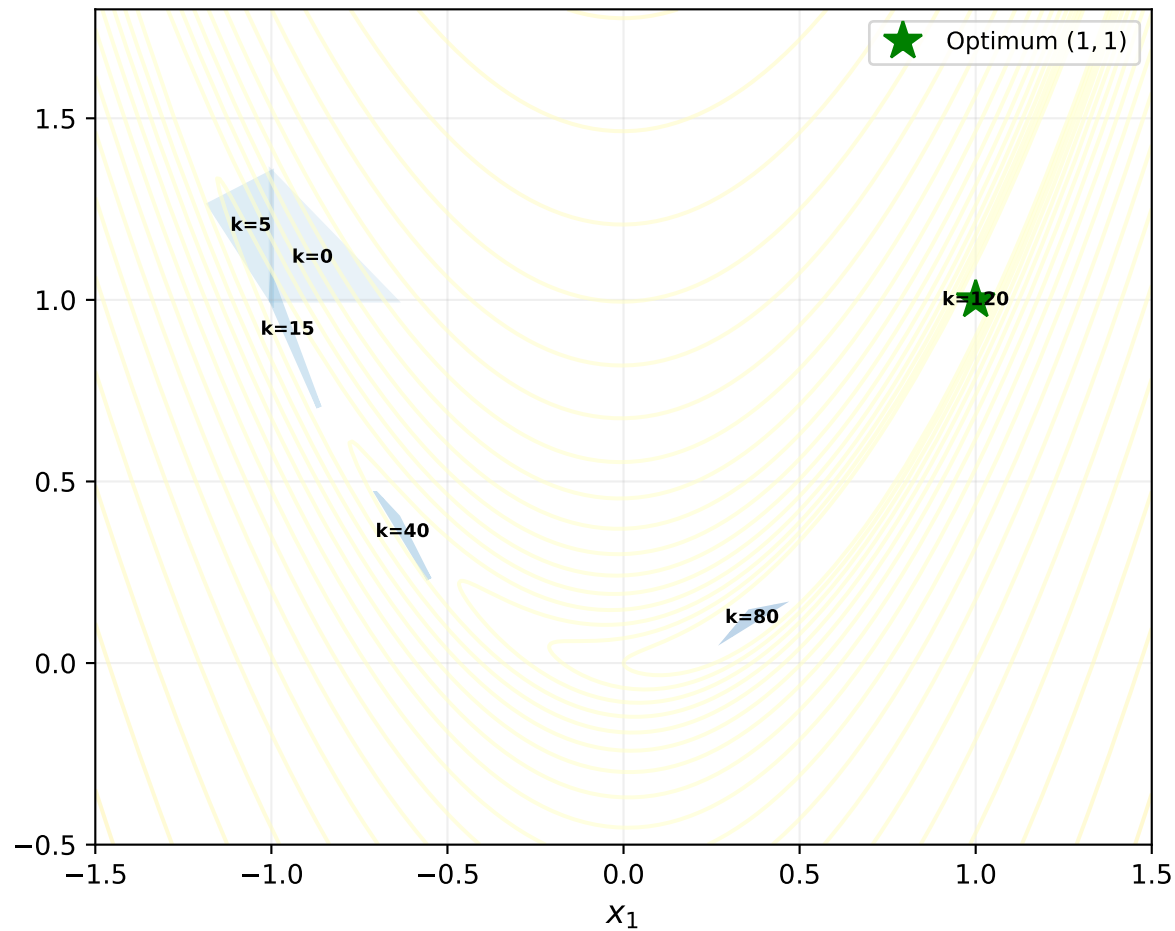
Nelder--Mead Simplex Evolution (triangles at selected iterations)
