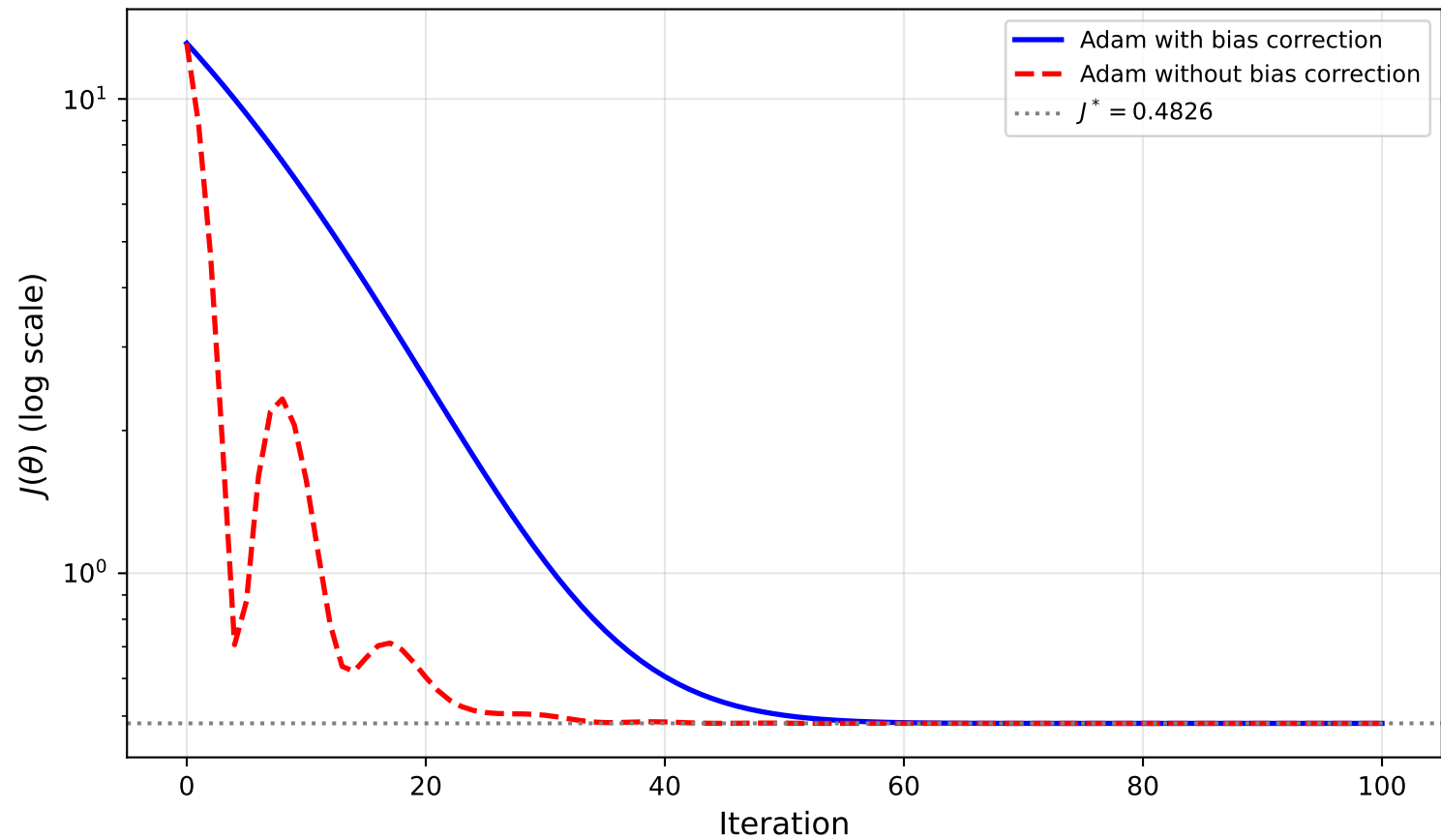
Adam: Effect of Bias Correction on Early Convergence (Benchmark A)
