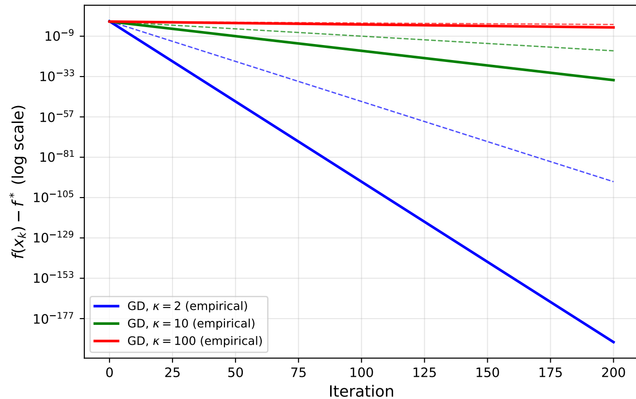
Effect of Condition Number on GD Convergence Rate (solid: empirical, dashed: theoretical ((\kappa - 1)/(\kappa + 1))^k )
