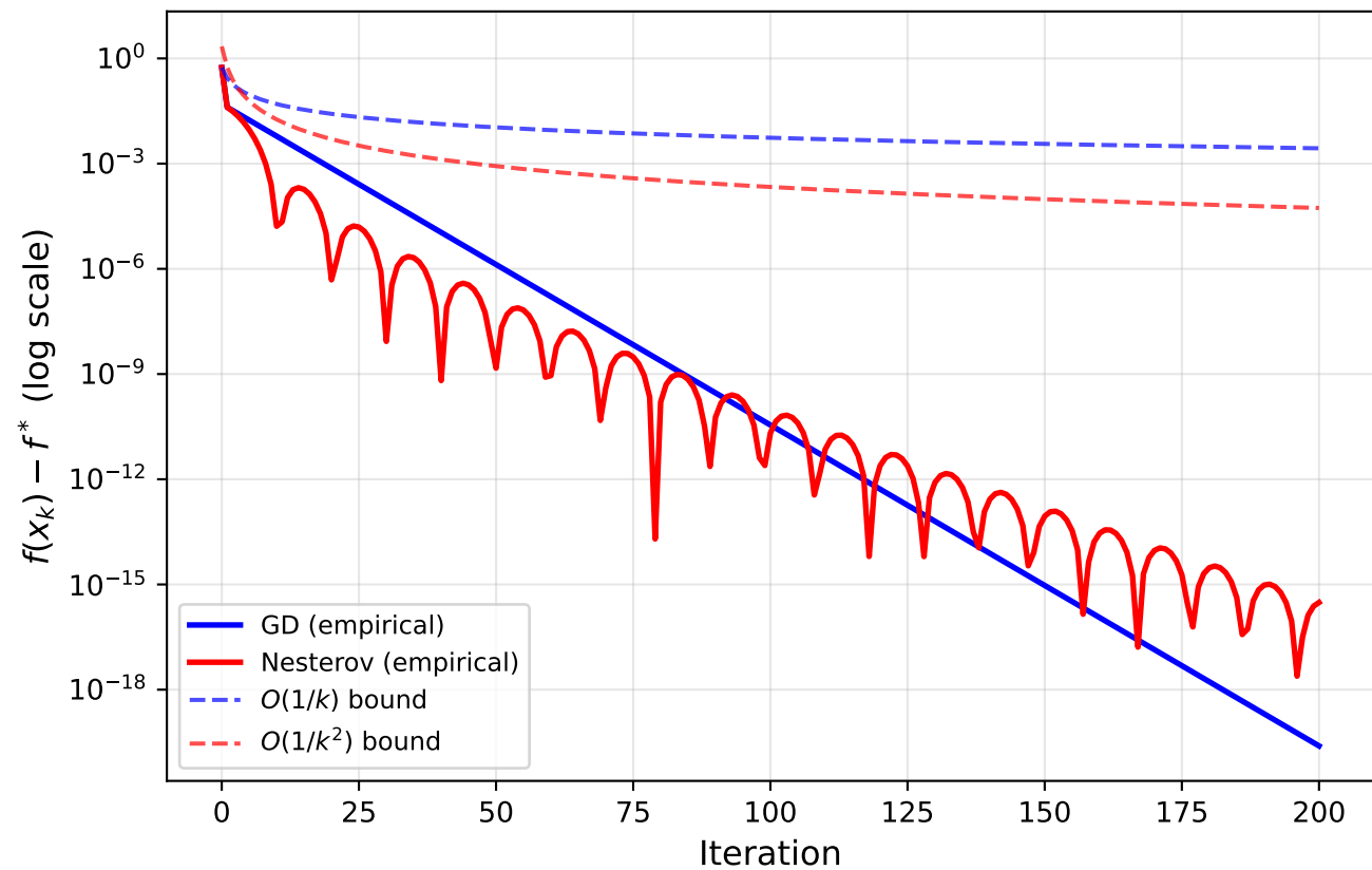
GD vs Nesterov: Empirical vs Theoretical Rates ( \kappa = 10 quadratic, \alpha = 1/L )
