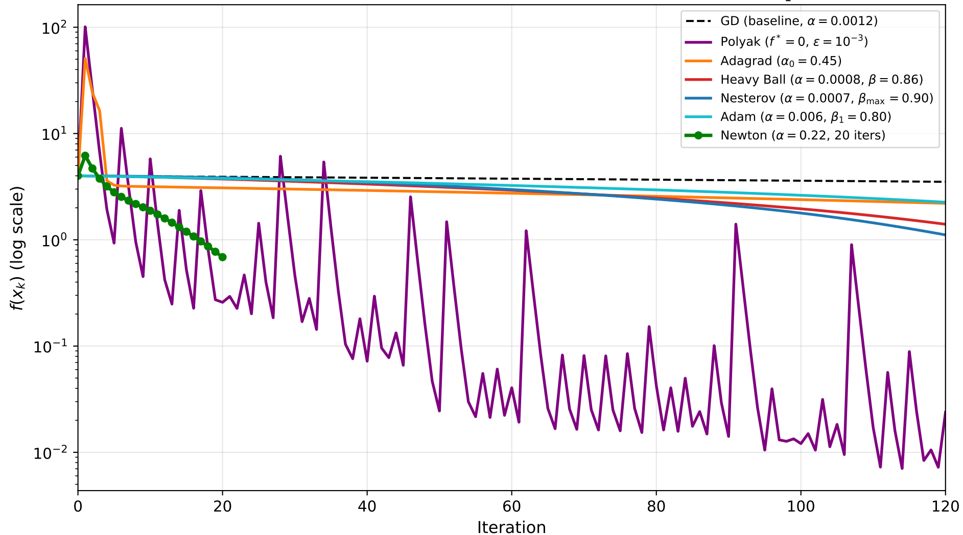
Cross-Method Comparison on Rosenbrock f(x) = (1 - x_1)^2 + 100(x_2 - x_1^2)^2
