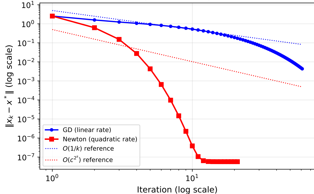
Log-Log: Linear vs Quadratic Convergence (Benchmark B)
