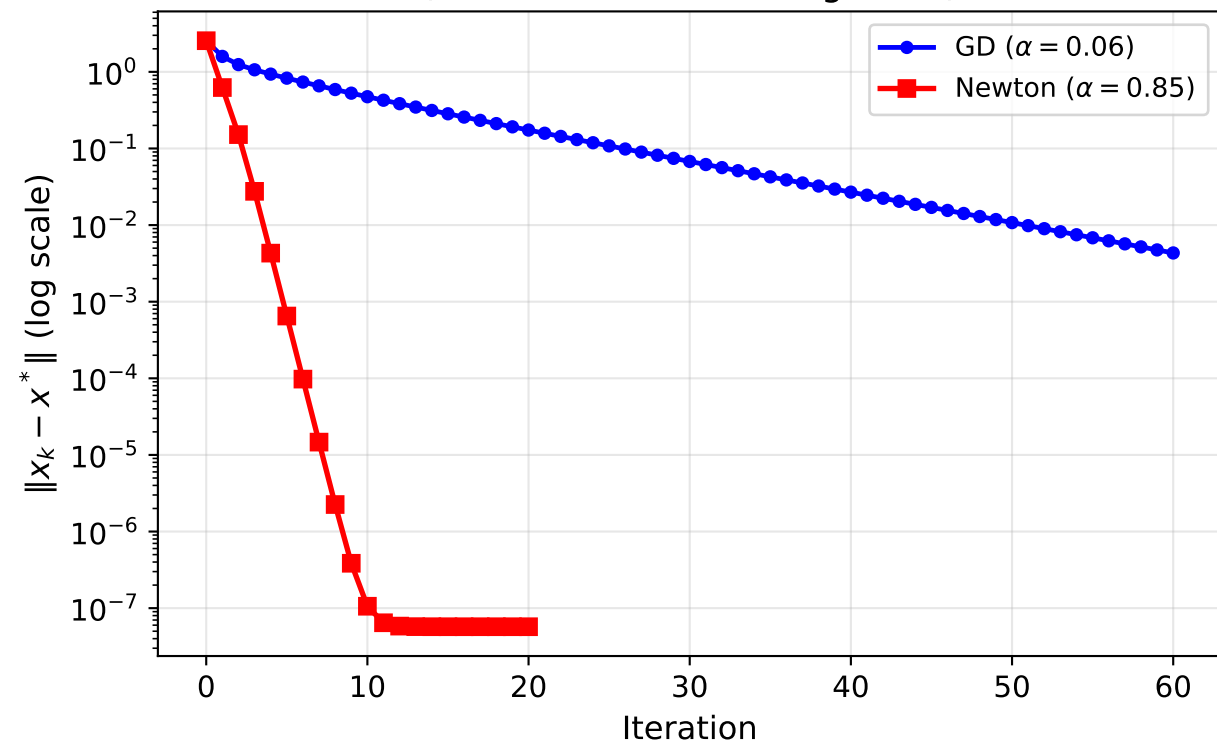
Distance to Optimum vs Iteration (Benchmark B, semi-log scale)
