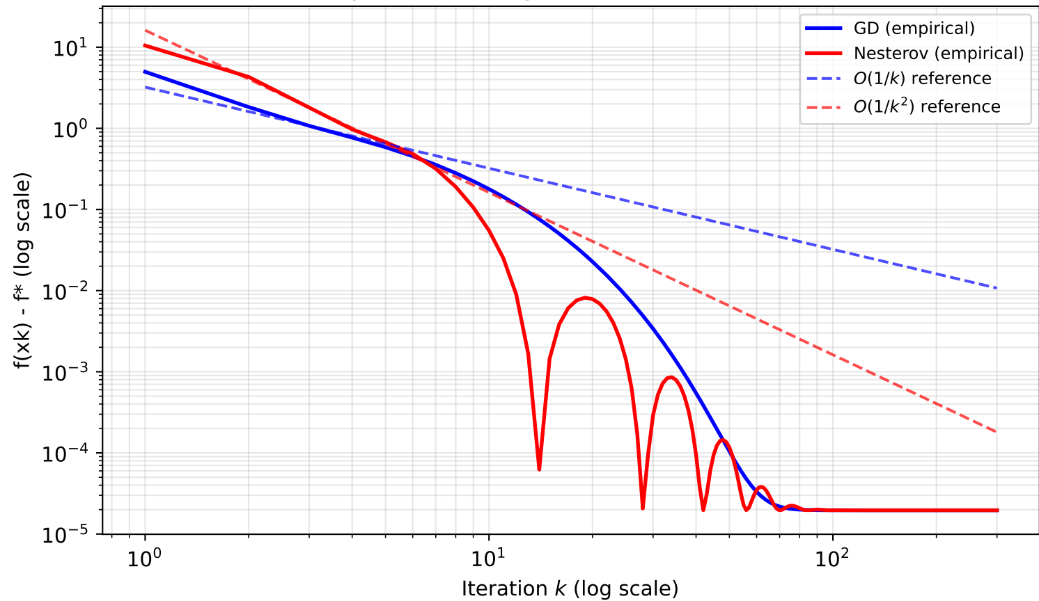
Q2: Empirical Convergence Rates on Benchmark B
