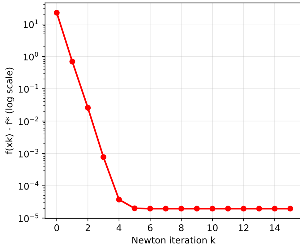
Benchmark B (Toy NN)
