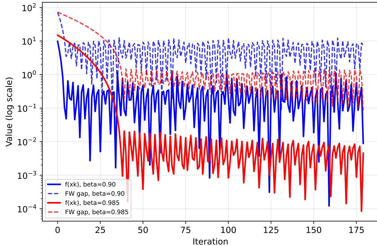
Q6-II: FW Objective and FW Gap
