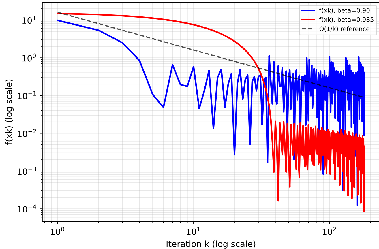
Q6-II: FW Rate (log-log)
