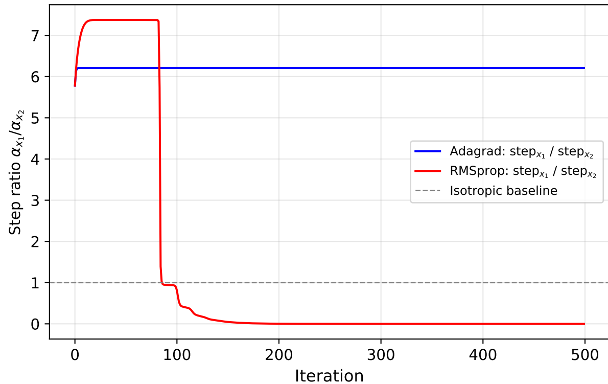
Coordinate Adaptation: Step-Size Ratio (ratio > 1: more steps in x_1 direction)
