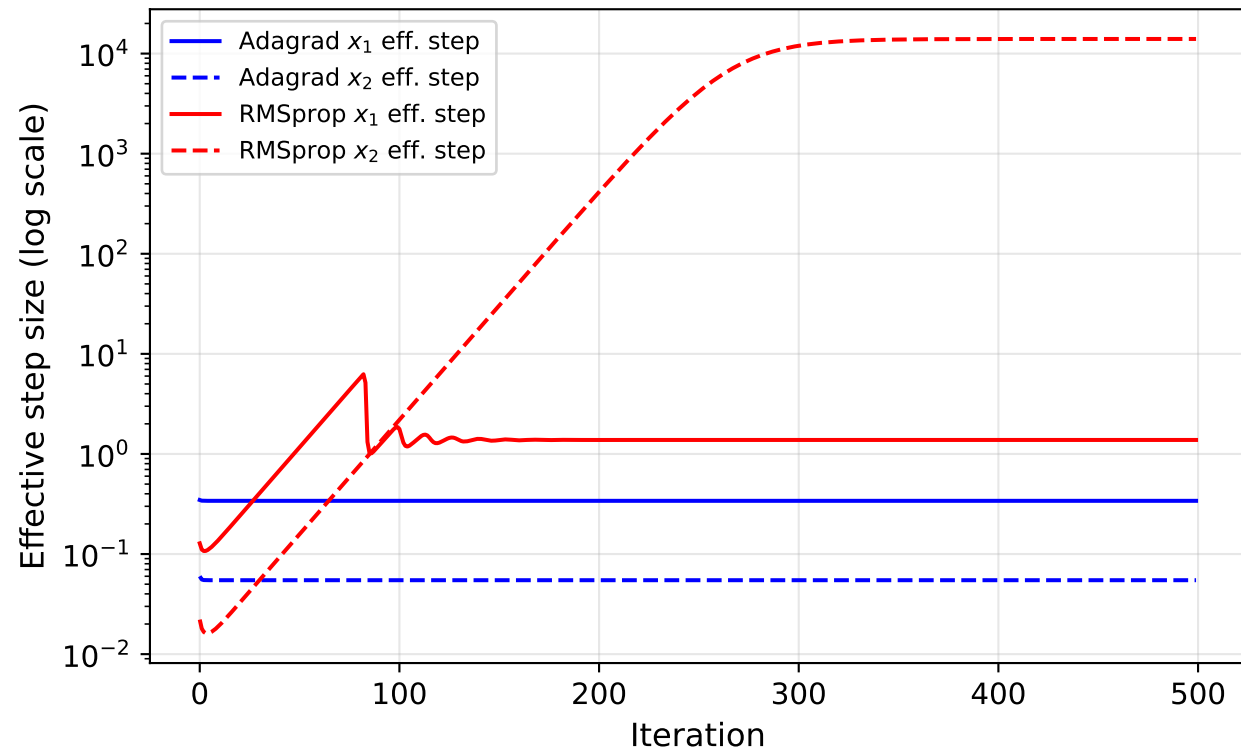
Adagrad vs RMSprop: Per-Coordinate Effective Step (Benchmark B, 500 iterations)
