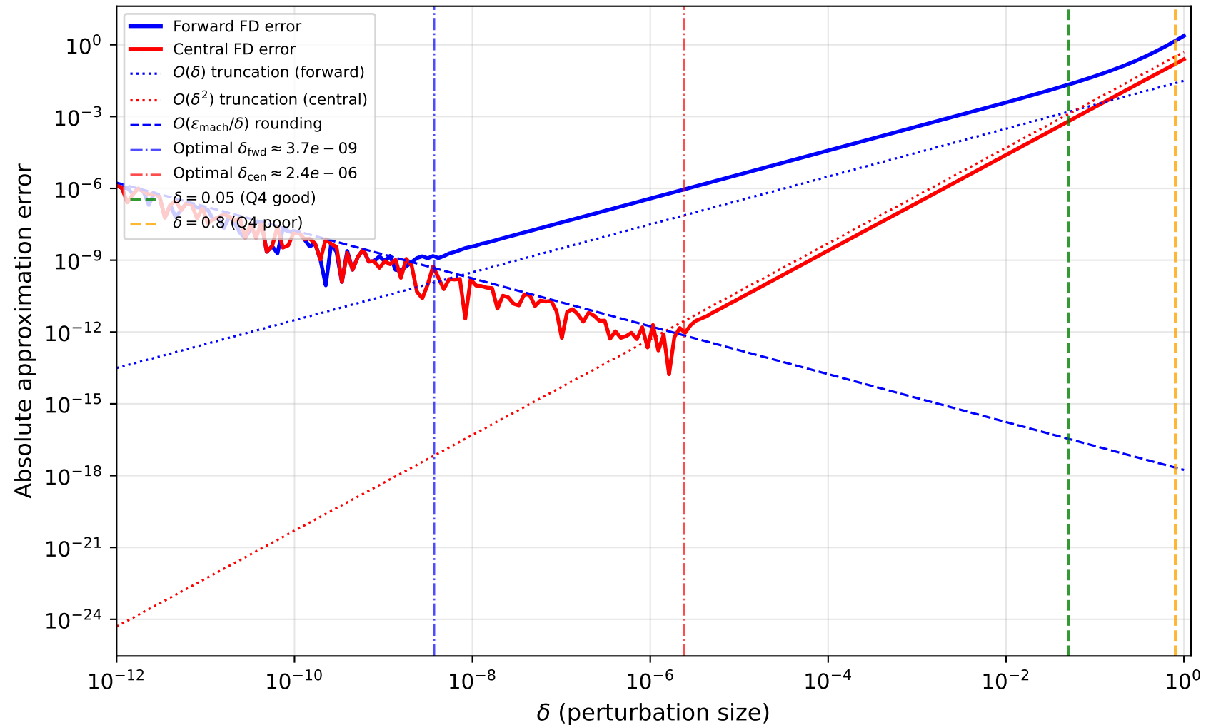
Finite Difference Approximation Error for g(x) = x^4 at x_0 = 0.25 (Forward vs Central Differences)
