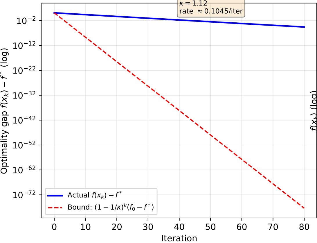
Benchmark A: Actual vs Theoretical Bound ( \kappa = 1.12, \alpha = 0.08 )
