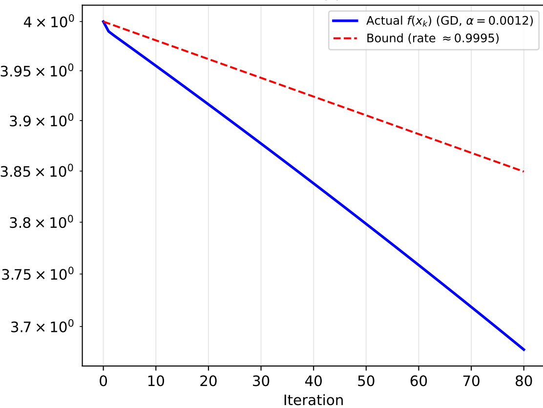
Benchmark C: GD Stagnation on Rosenbrock ( \alpha = 0.0012, L_{\text{start}} \approx 1002 )
