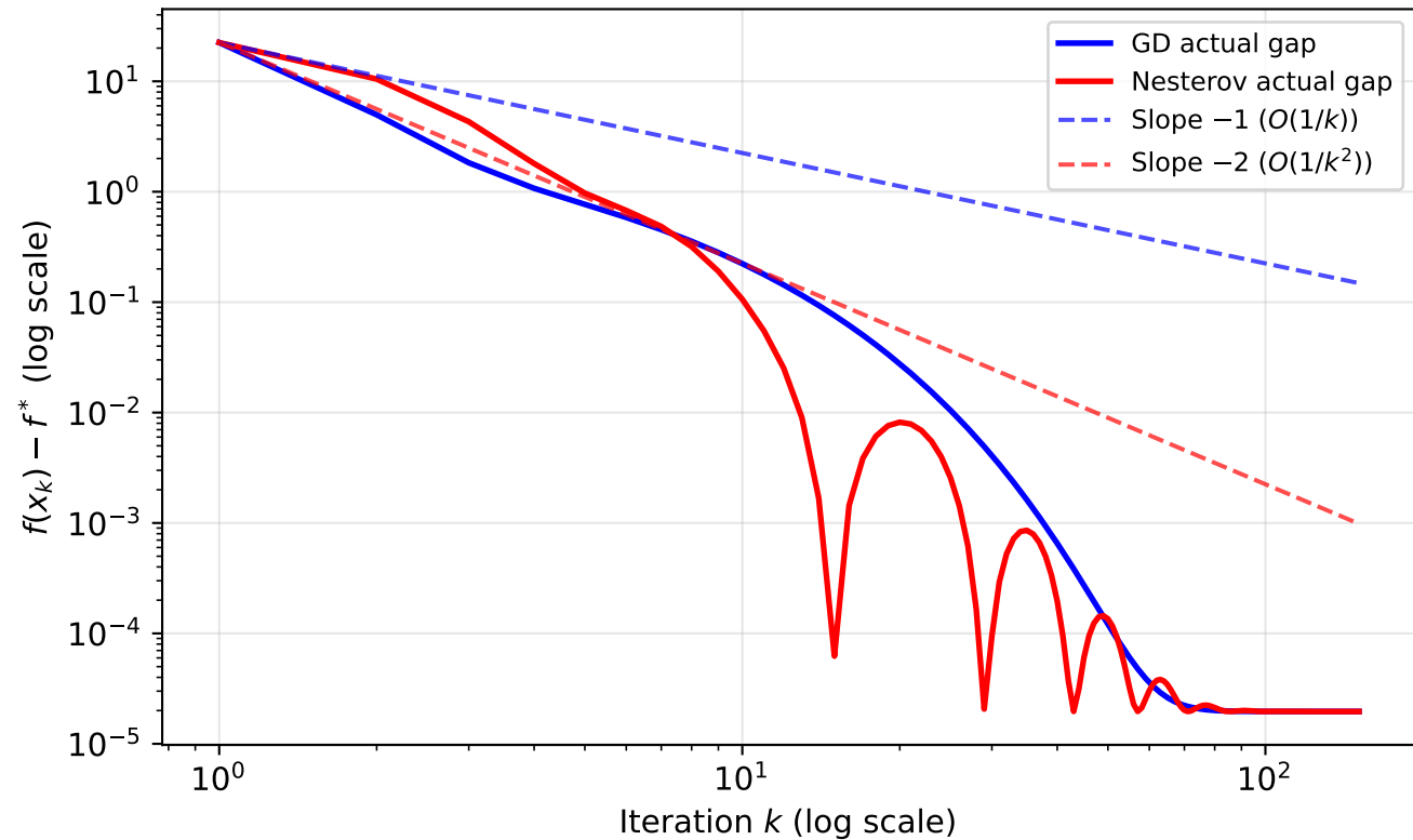
Log-Log Plot: Nesterov Rate is O(1/k^2)
