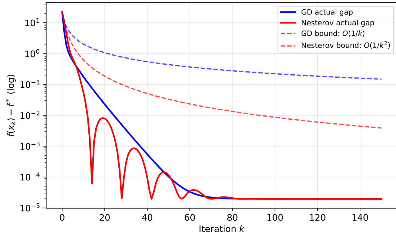
Benchmark B: O(1/k) vs O(1/k^2) Convergence
