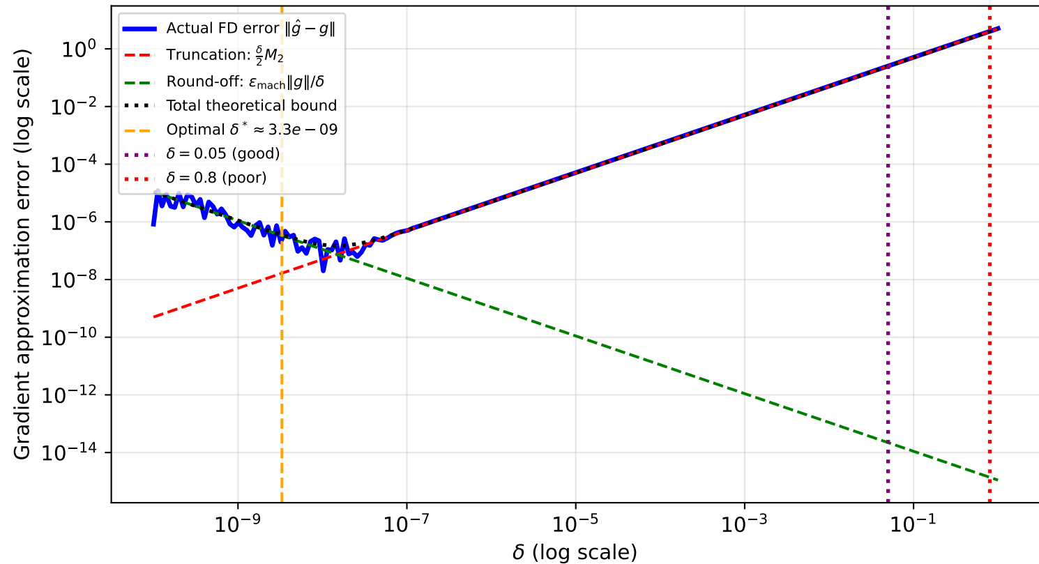
Q4: Forward Finite-Difference Error vs Step Size \delta (Benchmark B at x = (0, 3) )
