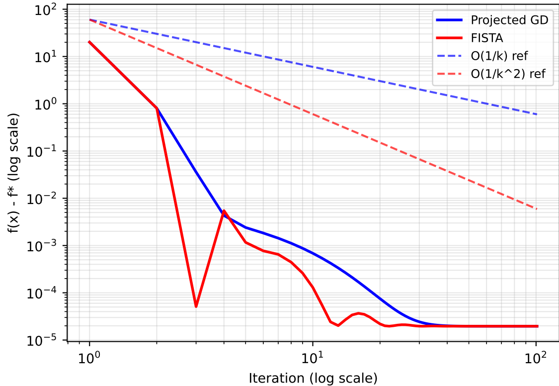
Log-log convergence rate comparison
