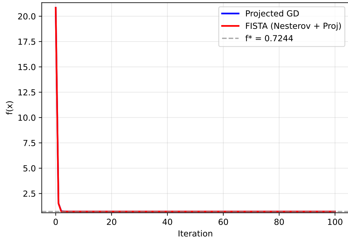
Q5: PGD vs FISTA convergence (Benchmark B, x_1 \geq 0.5 )
